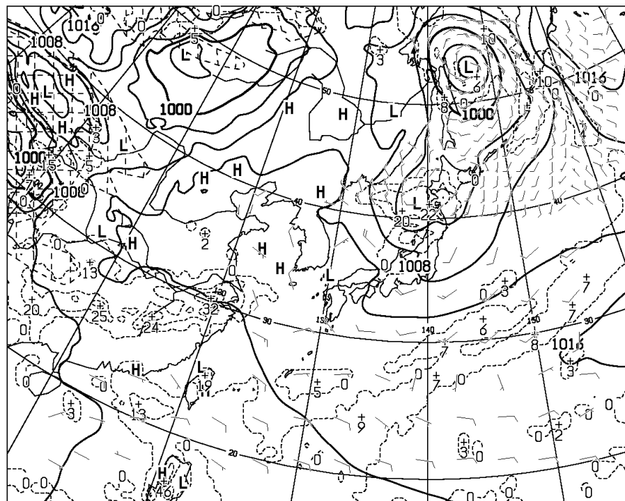
T=24 VALID 201200UTC SURFACE PRESS (hPa), PRECIP (MM) (12-24) WIND ARROW AT SURFACE
