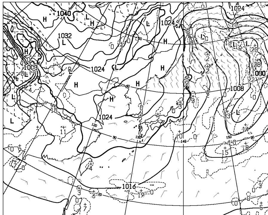
T=24 VALID 141200UTC SURFACE PRESS(hPa), PRECIP(MM) (12-24) WIND ARROW AT SURFACE
