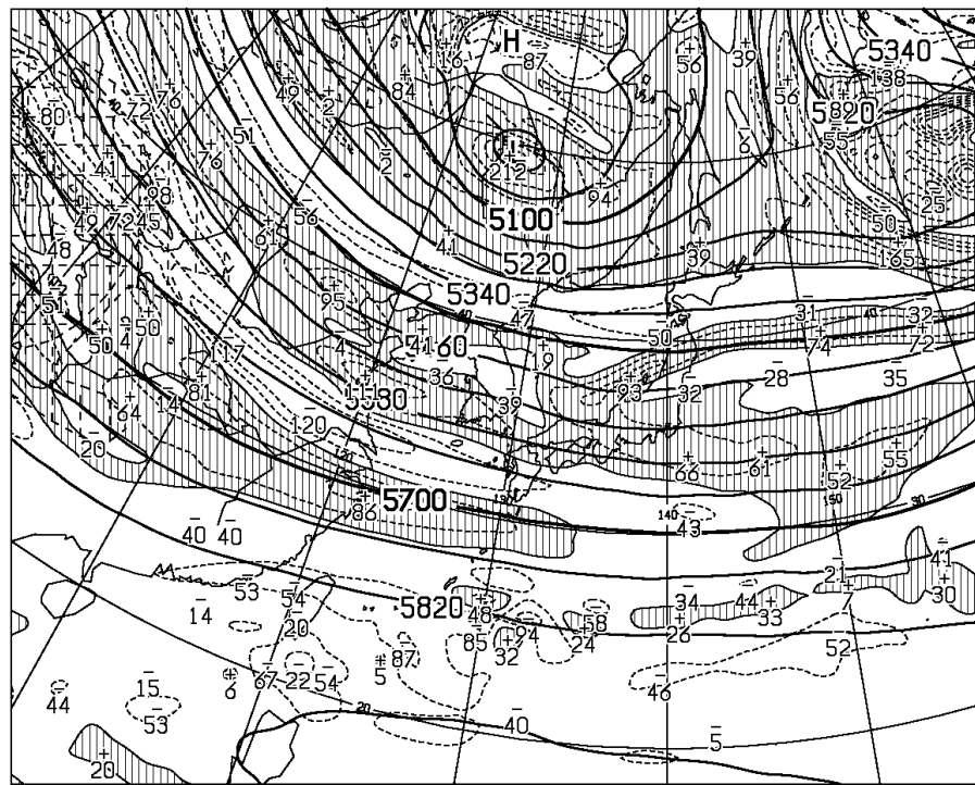
T=24 VALID 200000UTC HEIGHT (M), VORT (10**--6/SEC) AT 500hPa
