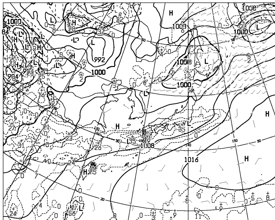
T=24 VALID 231200UTC SURFACE PRESS (hPa), PRECIP (MM) (12-24) WIND ARROW AT SURFACE
