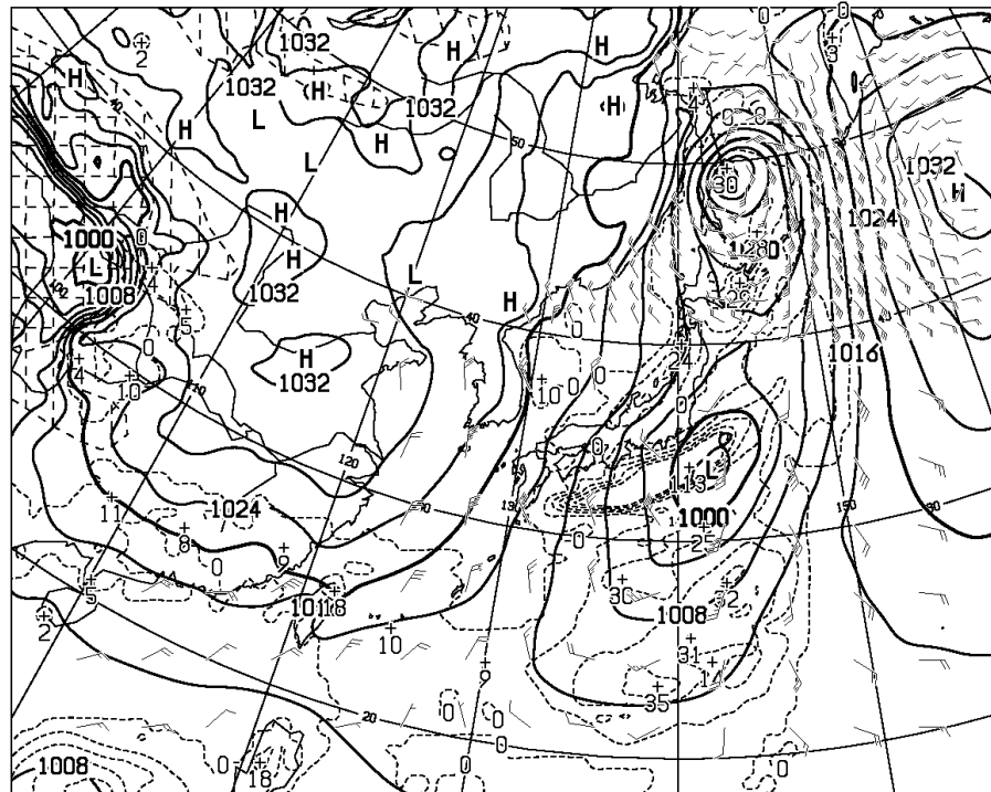
T=24 VALID 181200UTC SURFACE PRESS (hPa), PRECIP (MM) (12-24) WIND ARROW AT SURFACE
