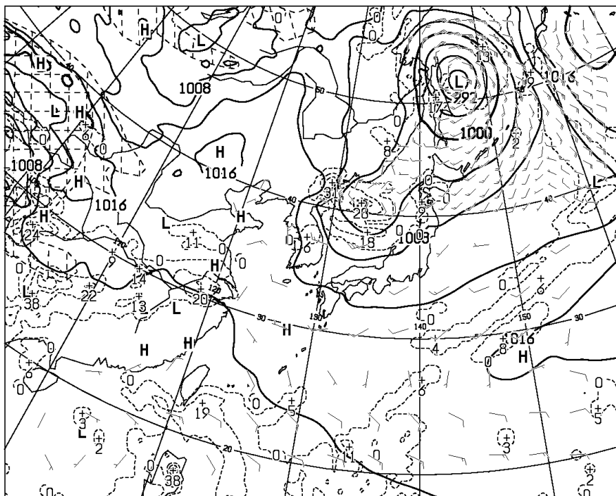
T=12 VALID 200000UTC SURFACE PRESS (hPa), PRECIP (MM) (00-12) WIND ARROW AT SURFACE
