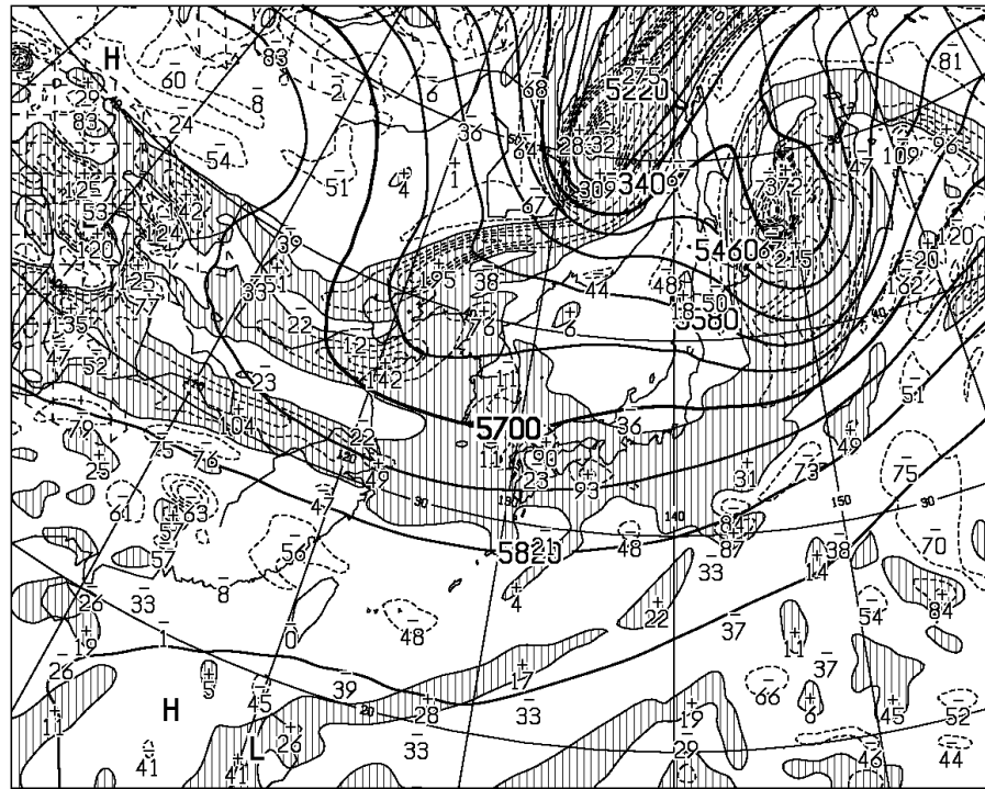
T=24 VALID 261200UTC HEIGHT (M), VORT (10**-6/SEC) AT 500hPa
