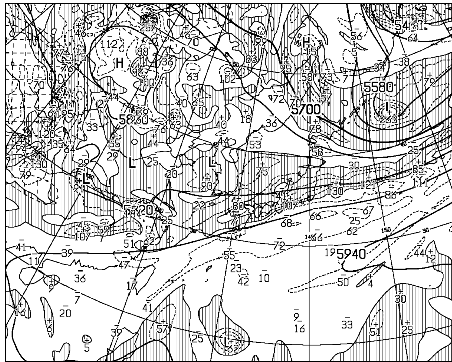
T=24 VALID 280000UTC HEIGHT (M), VORT (10**--6/SEC) AT 500hPa
