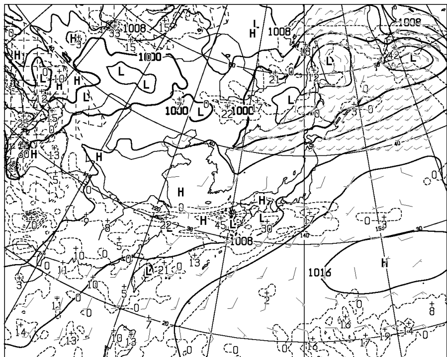
T=12 VALID 230000UTC SURFACE PRESS (hPa), PRECIP (MM) (00-12) WIND ARROW AT SURFACE
