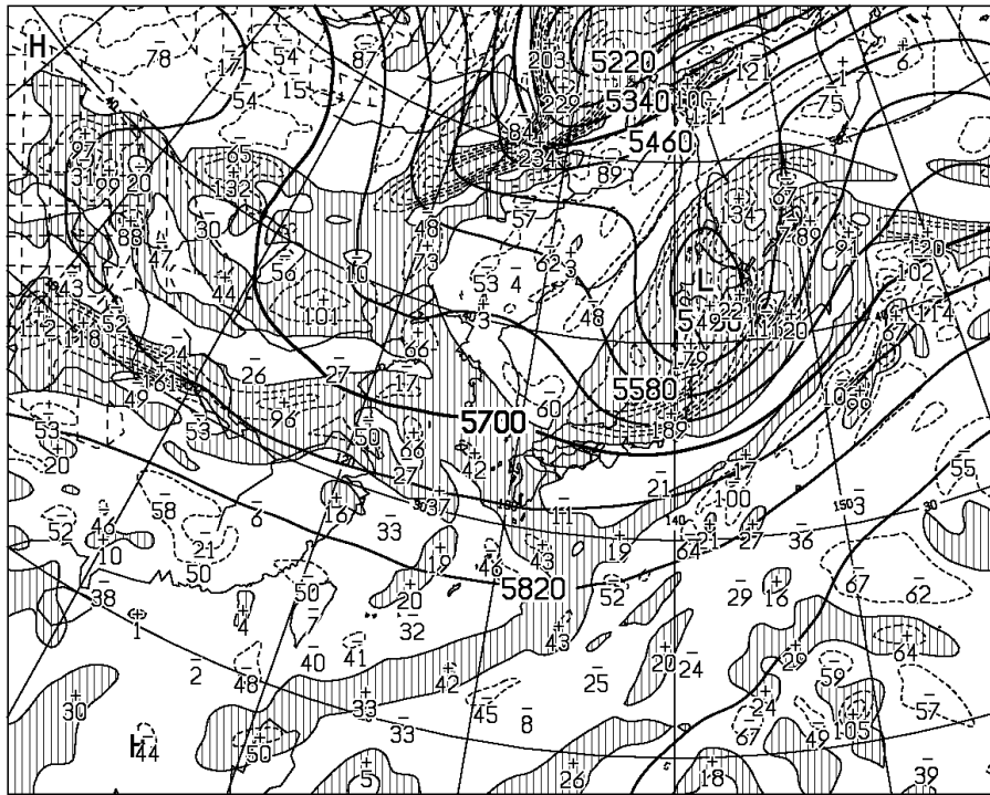
T=12 VALID 260000UTC HEIGHT (M), VORT (10**-6/SEC) AT 500hPa
