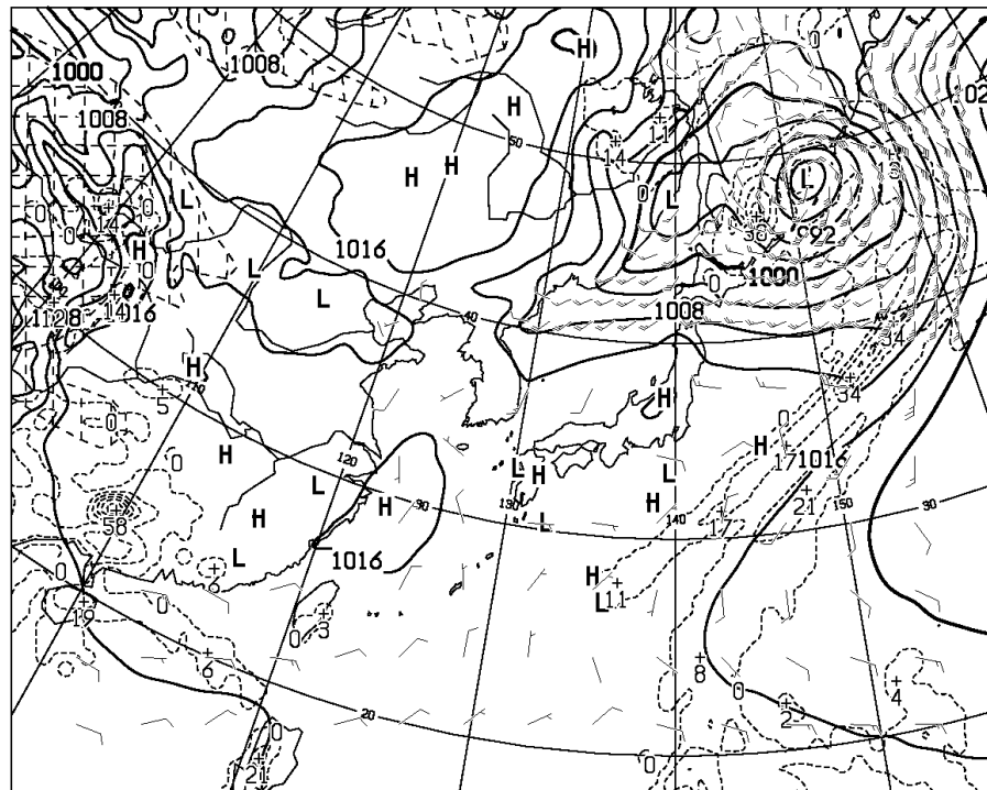
T=24 VALID 261200UTC SURFACE PRESS (hPa), PRECIP (MM) (12-24) WIND ARROW AT SURFACE
