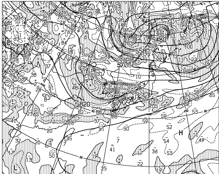
T=12 VALID 230000UTC HEIGHT (M), VORT (10** \times -6/SEC) AT 500hPa
