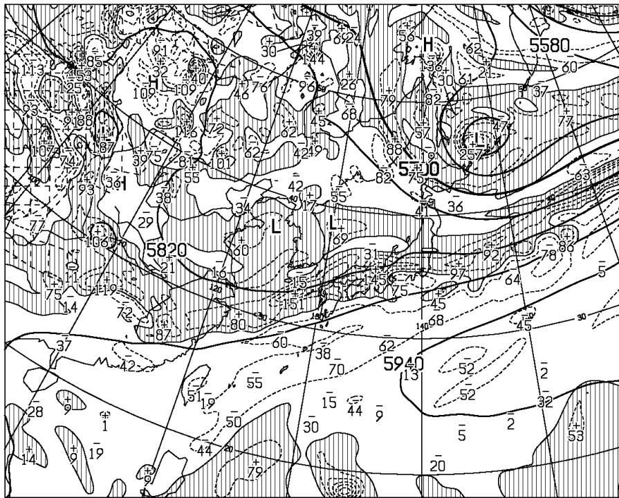
T=12 VALID 271200UTC HEIGHT (M), VORT (10**--6/SEC) AT 500hPa
