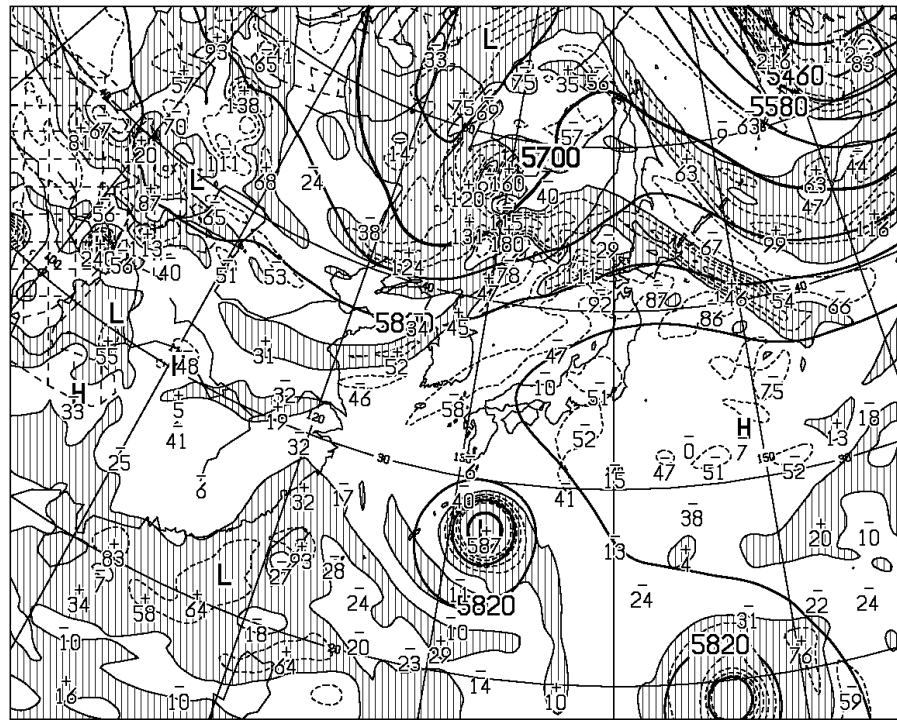
T=24 VALID 210000UTC HEIGHT (M), VORT(10**-6/SEC) AT 500hPa
