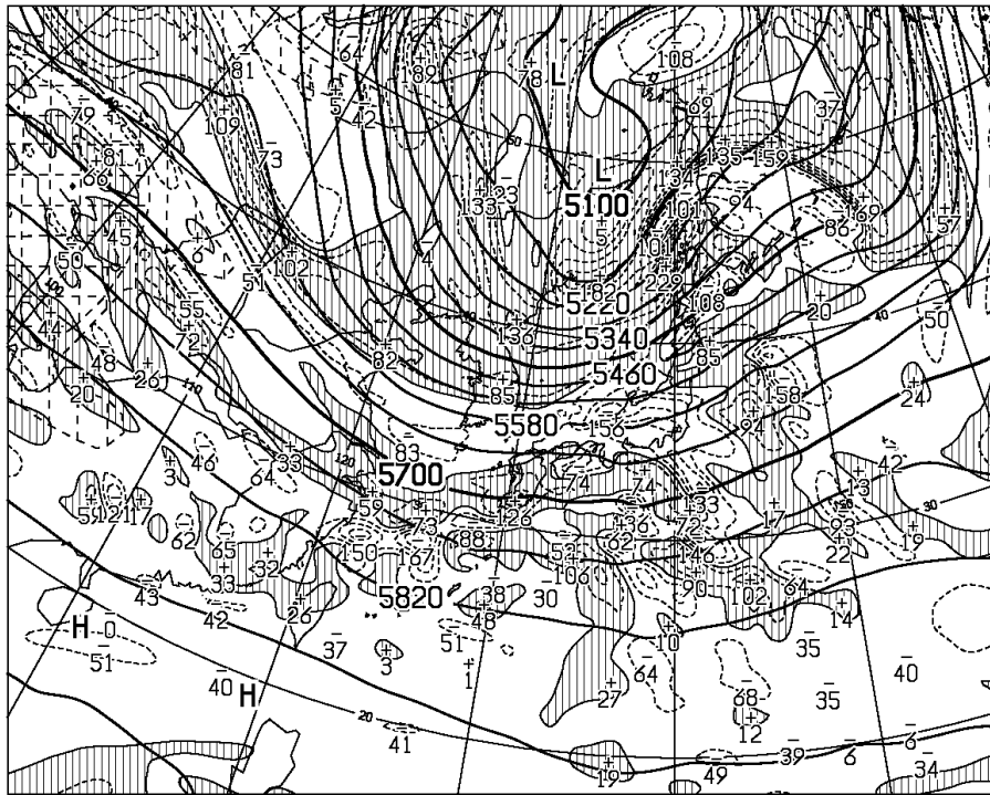
T=12 VALID 180000UTC HEIGHT (M), VORT (10** \frac{-6}{\text{SEC}} ) AT 500hPa
