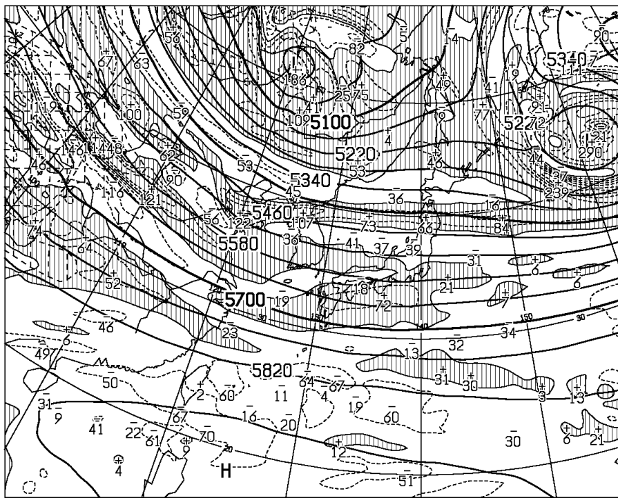
T=12 VALID 191200UTC HEIGHT (M), VORT (10**--6/SEC) AT 500hPa
