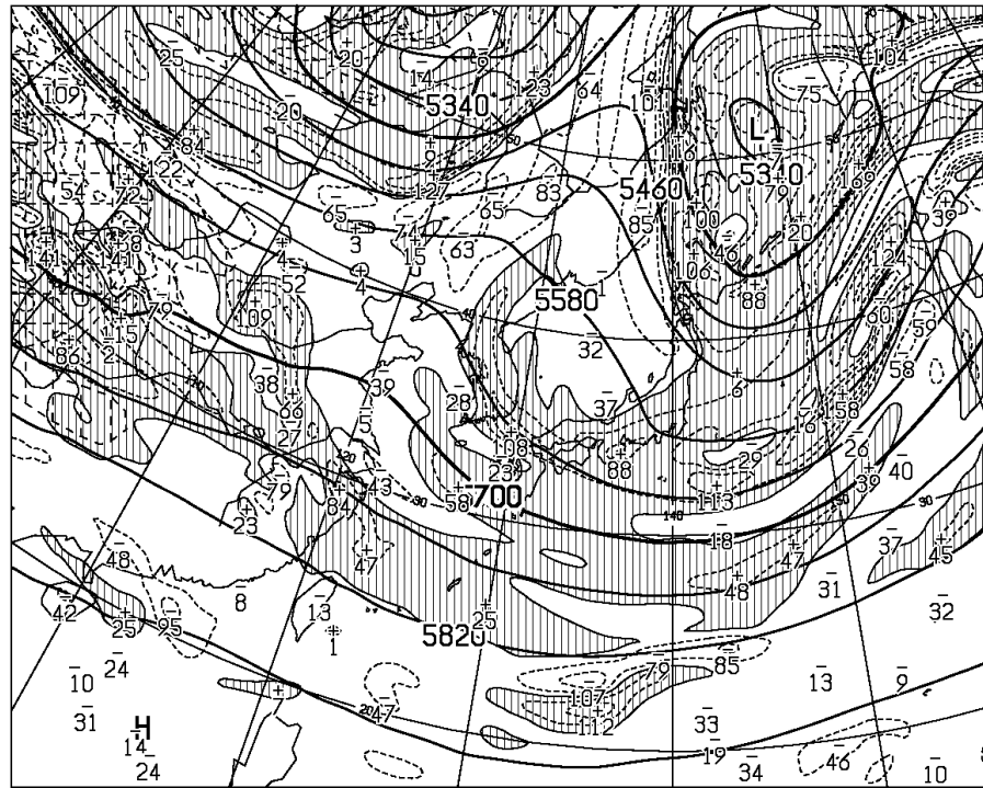
T=24 VALID 141200UTC HEIGHT (M), VORT(10** \times -6/SEC) AT 500hPa
