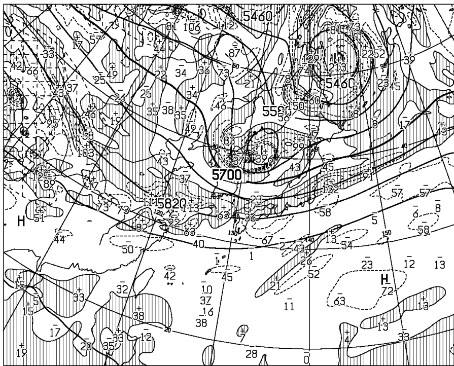
T=12 VALID 200000UTC HEIGHT (M), VORT (10** -6 /SEC) AT 500hPa
