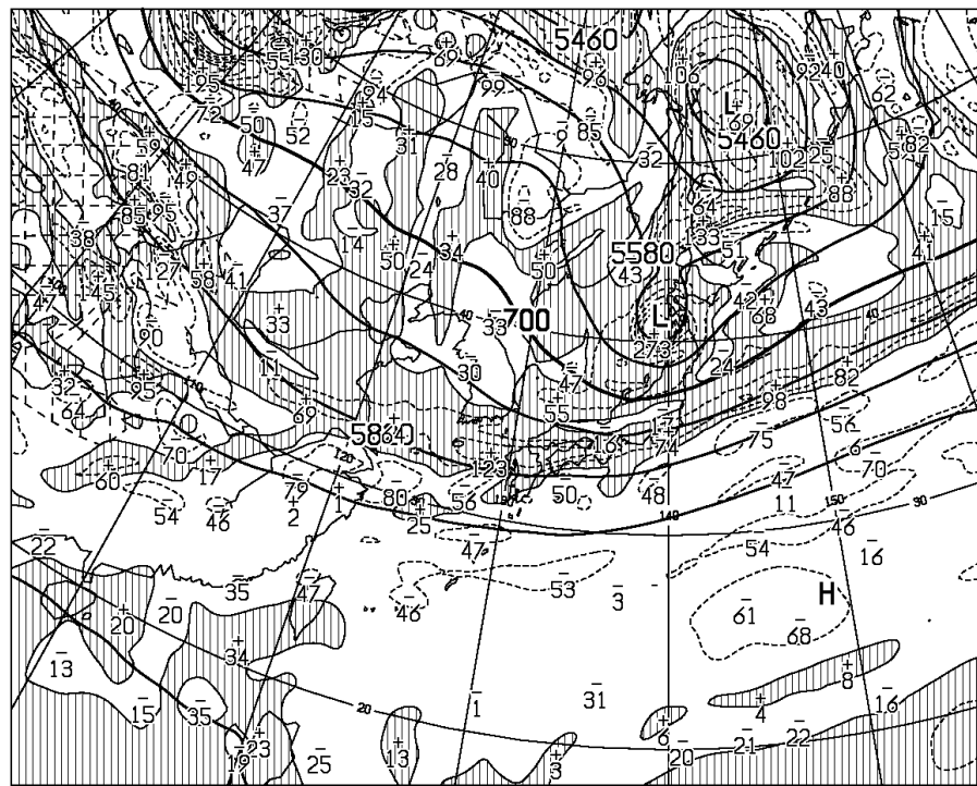
T=24 VALID 201200UTC HEIGHT (M), VORT (10** -6 /SEC) AT 500hPa
