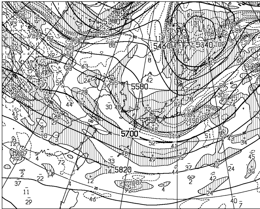
T=12 VALID 140000UTC HEIGHT (M), VORT(10** \times -6/SEC) AT 500hPa
