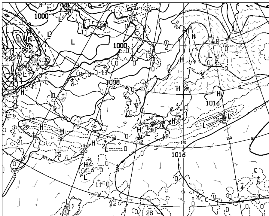
T=12 VALID 271200UTC SURFACE PRESS (hPa), PRECIP (MM) (00-12) WIND ARROW AT SURFACE
