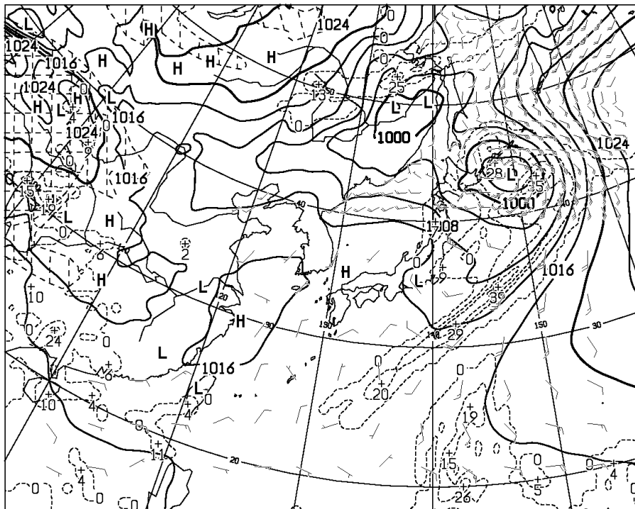
T=12 VALID 260000UTC SURFACE PRESS (hPa), PRECIP (MM) (00-12) WIND ARROW AT SURFACE
