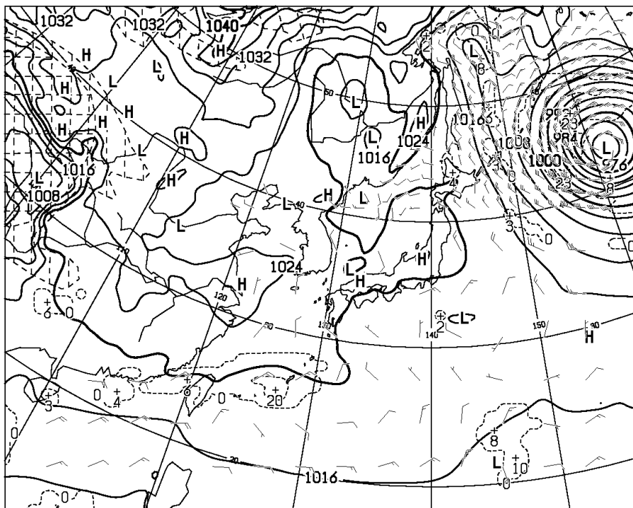
T=12 VALID 191200UTC SURFACE PRESS (hPa), PRECIP (MM) (00-12) WIND ARROW AT SURFACE
