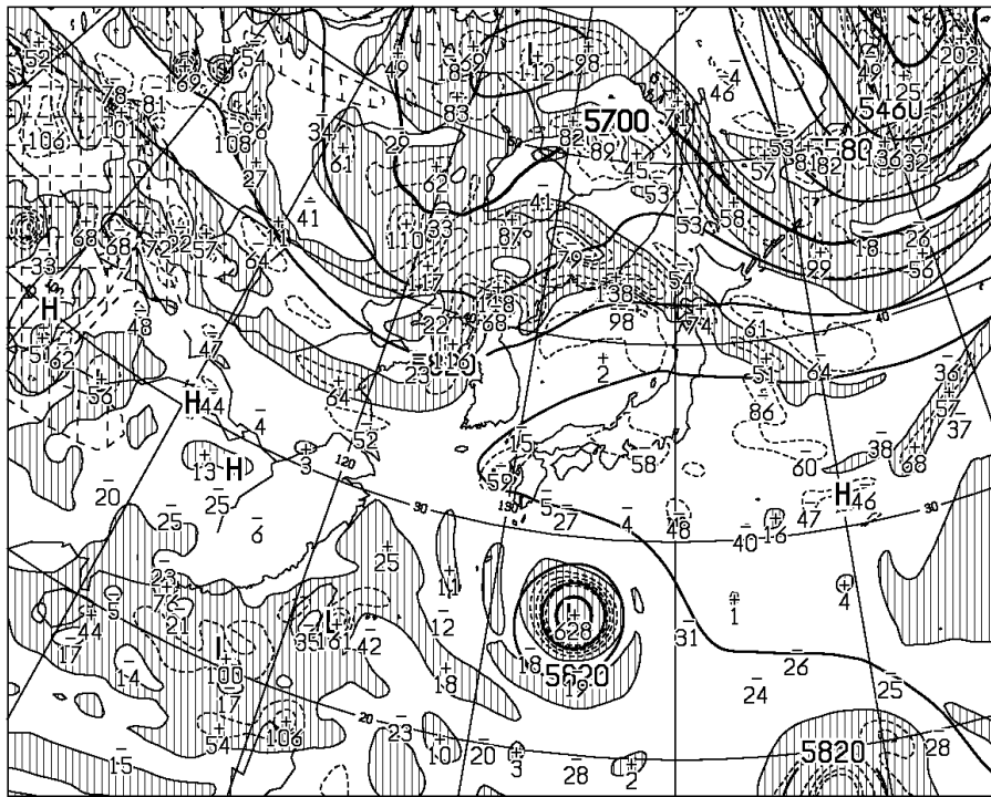
T=12 VALID 201200UTC HEIGHT (M), VORT(10**-6/SEC) AT 500hPa
