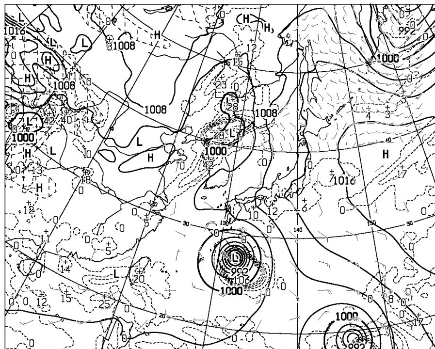
T=24 VALID 210000UTC SURFACE PRESS(hPa), PRECIP (MM) (12-24) WIND ARROW AT SURFACE
