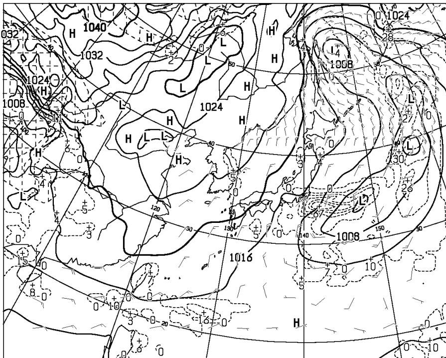
T=12 VALID 140000UTC SURFACE PRESS(hPa), PRECIP(MM) (00-12) WIND ARROW AT SURFACE
