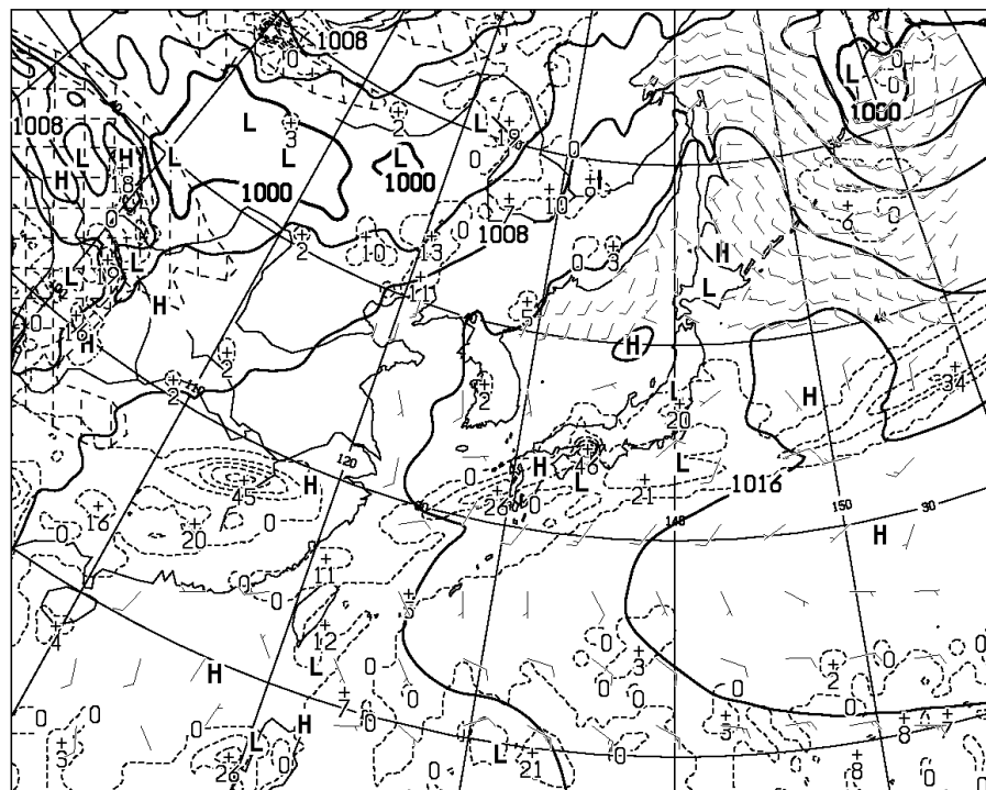
T=24 VALID 280000UTC SURFACE PRESS (hPa), PRECIP (MM) (12-24) WIND ARROW AT SURFACE
