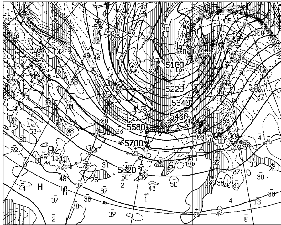
T=24 VALID 181200UTC HEIGHT (M), VORT (10** \frac{-6}{\text{SEC}} ) AT 500hPa
