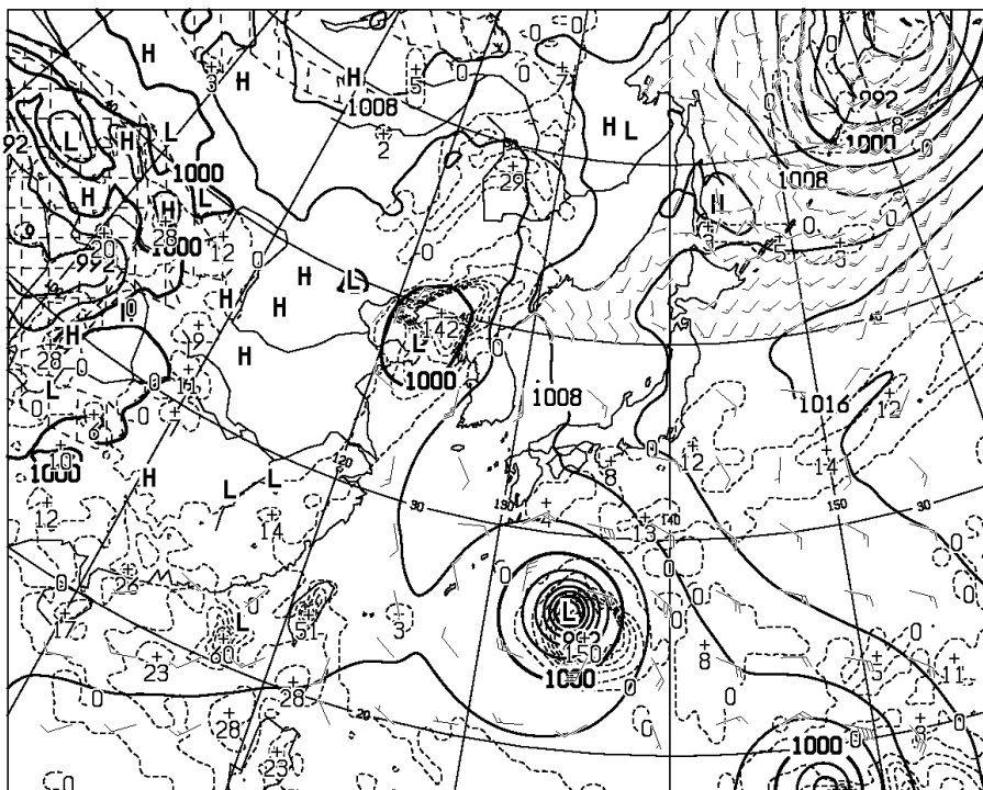
T=12 VALID 201200UTC SURFACE PRESS(hPa), PRECIP (MM) (00-12) WIND ARROW AT SURFACE
