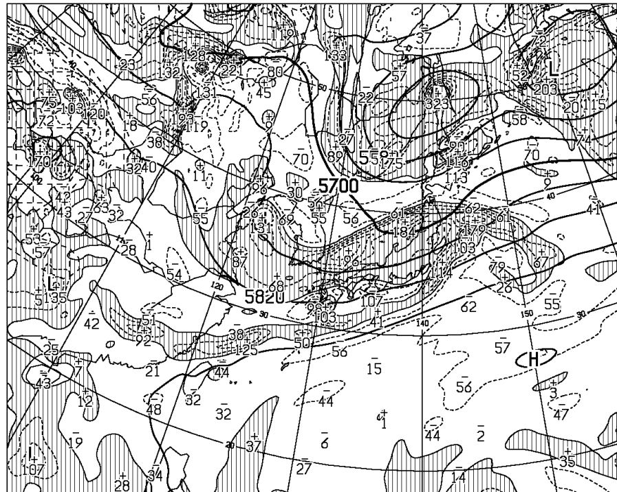
T=24 VALID 231200UTC HEIGHT (M), VORT (10** \times -6/SEC) AT 500hPa
