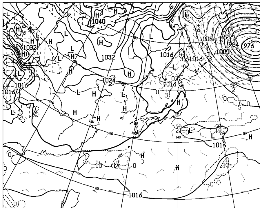
T=24 VALID 200000UTC SURFACE PRESS (hPa), PRECIP (MM) (12-24) WIND ARROW AT SURFACE
