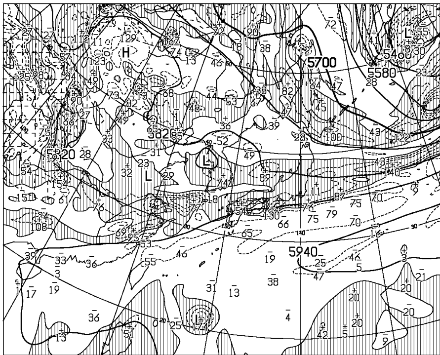
T=36 VALID 281200UTC HEIGHT (M), VORT (10 -6 /SEC) AT 500hPa
