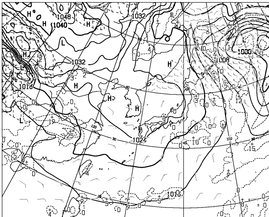
T=36 VALID 150000UTC SURFACE PRESS (hPa), PRECIP (MM) (24-36) WIND ARROW AT SURFACE
