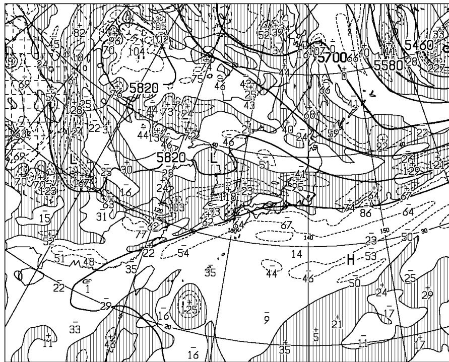
T=48 VALID 290000UTC HEIGHT (M), VORT (10 -6 /SEC) AT 500hPa
