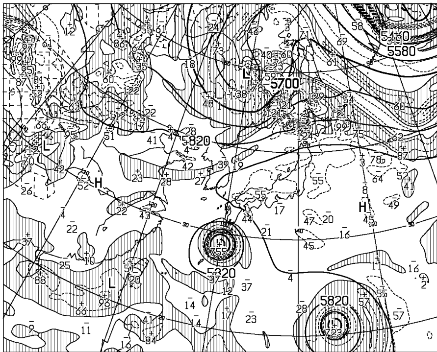
T=36 VALID 211200UTC HEIGHT (M), VORT (10** -6 /SEC) AT 500hPa
