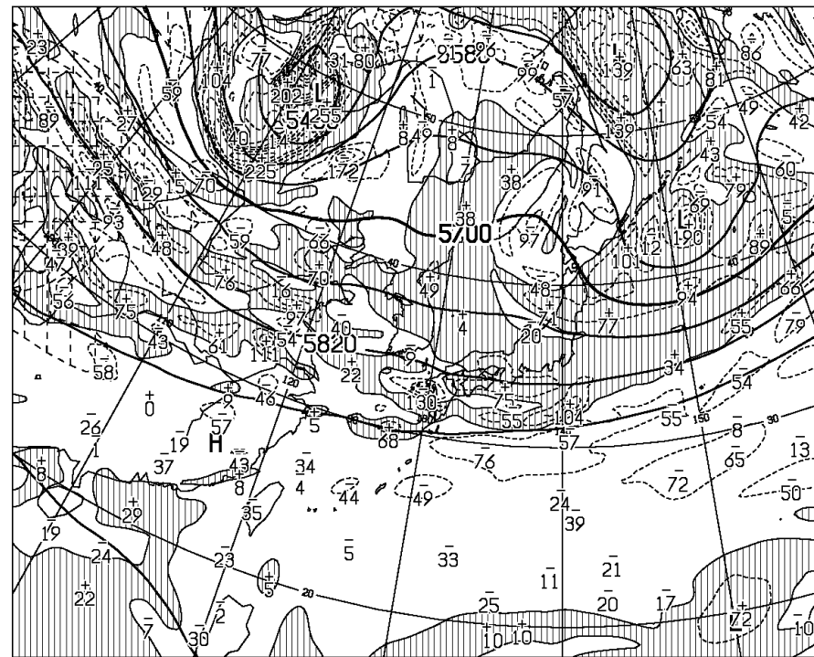
T=48 VALID 211200UTC HEIGHT (M), VORT (10** \times -6/SEC) AT 500hPa
