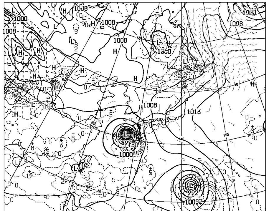
T=48 VALID 220000UTC SURFACE PRESS (hPa), PRECIP (MM) (36-48) WIND ARROW AT SURFACE
