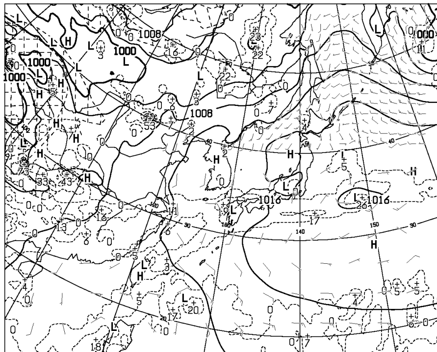
T=48 VALID 290000UTC SURFACE PRESS (hPa), PRECIP (MM) (36-48) WIND ARROW AT SURFACE
