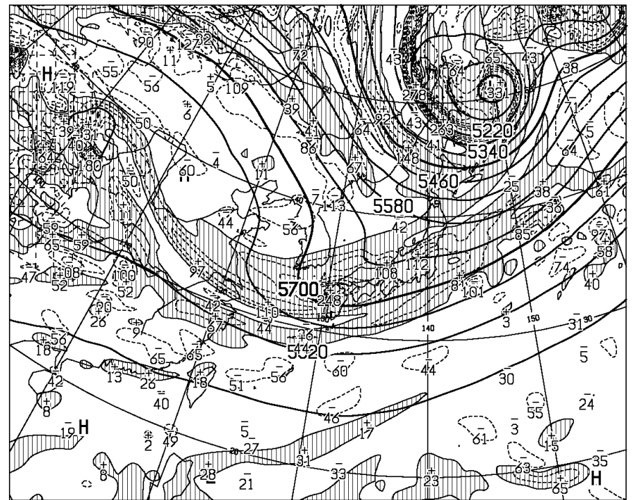
T=48 VALID 271200UTC HEIGHT (M), VORT (10**+6/SEC) AT 500hPa
