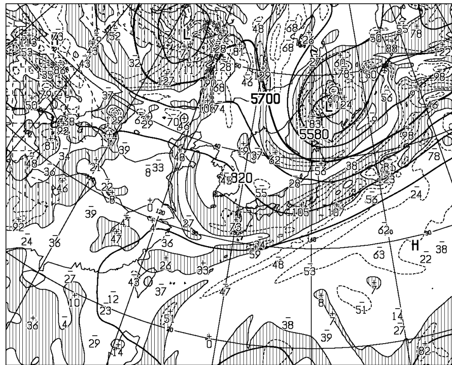
T=48 VALID 241200UTC HEIGHT (M), VORT (10**+6/SEC) AT 500hPa
