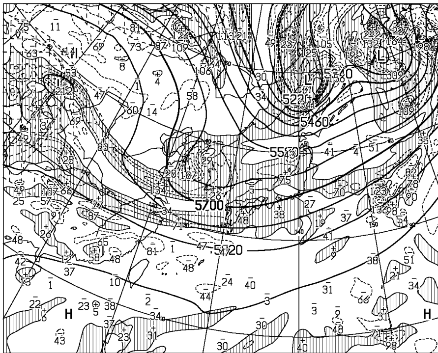
T=36 VALID 270000UTC HEIGHT (M), VORT (10**+6/SEC) AT 500hPa
