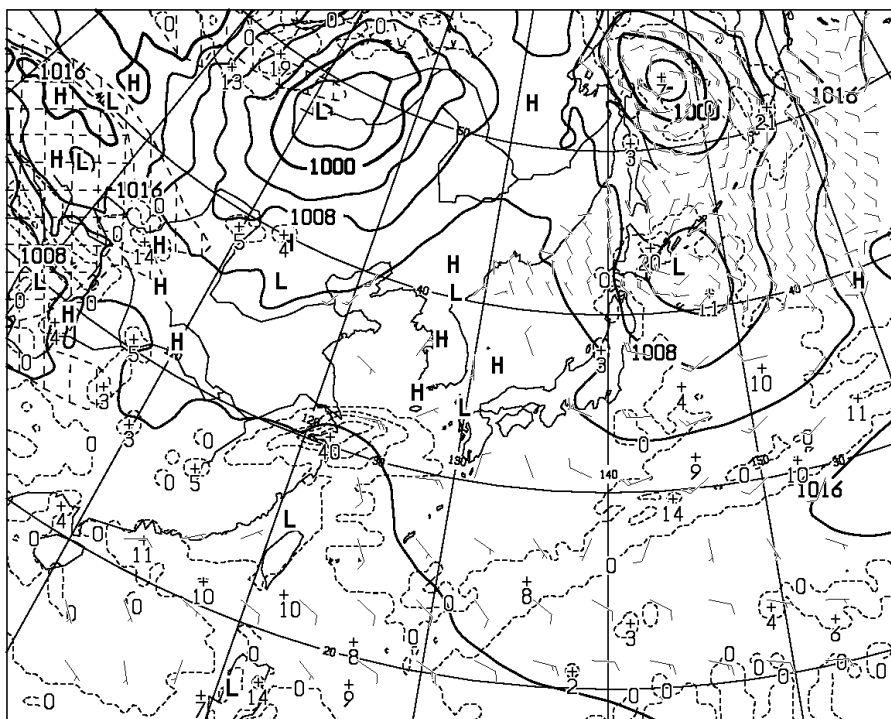
T=36 VALID 210000UTC SURFACE PRESS (hPa), PRECIP (MM) (24-36) WIND ARROW AT SURFACE
