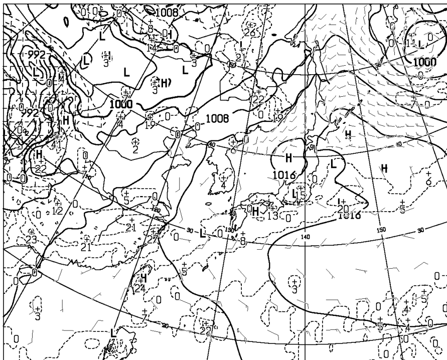
T=36 VALID 281200UTC SURFACE PRESS (hPa), PRECIP (MM) (24-36) WIND ARROW AT SURFACE
