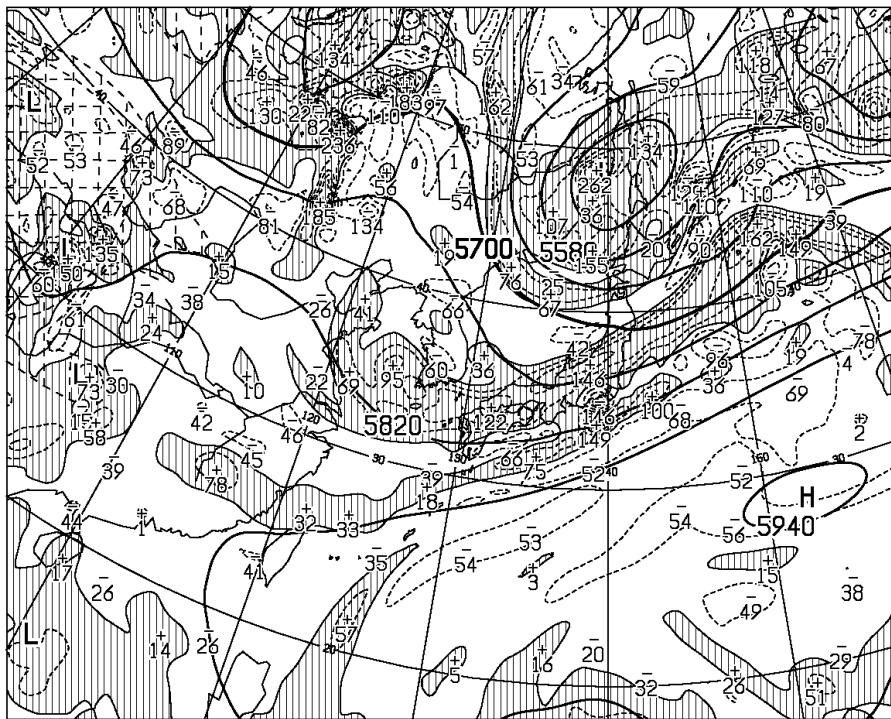
T=36 VALID 240000UTC HEIGHT (M), VORT (10**+6/SEC) AT 500hPa
