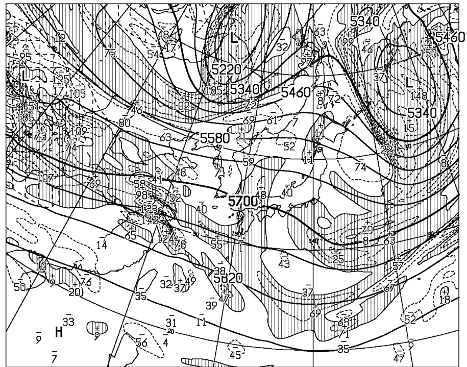
T=48 VALID 151200UTC HEIGHT (M), VORT (10 -6 /SEC) AT 500hPa
