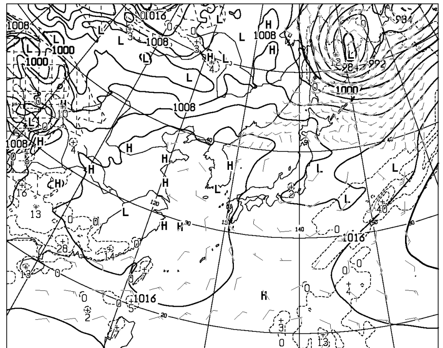
T=48 VALID 271200UTC SURFACE PRESS (hPa), PRECIP (MM) (36-48) WIND ARROW AT SURFACE
