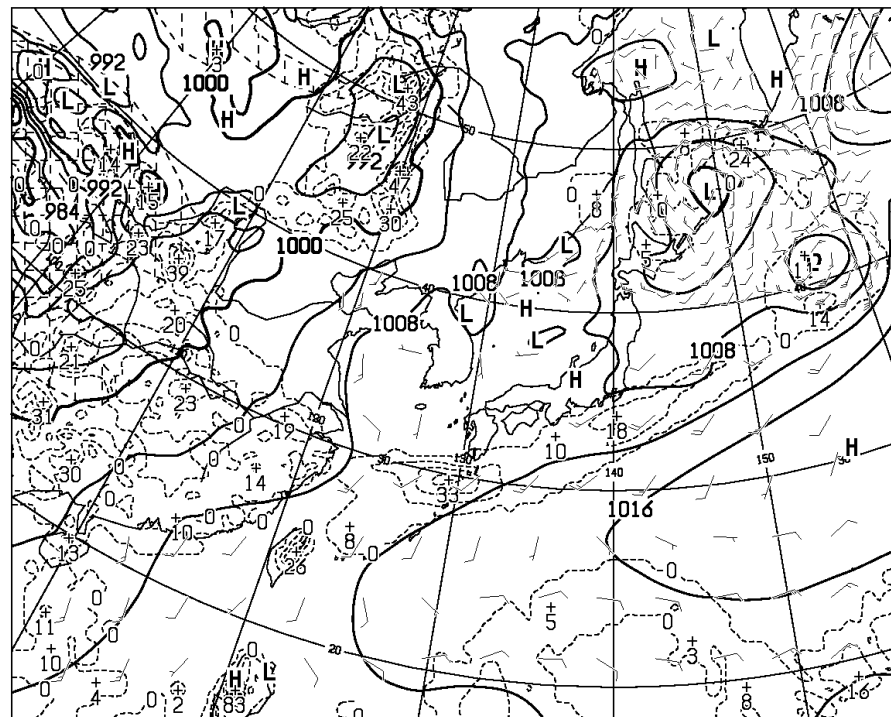
T=48 VALID 241200UTC SURFACE PRESS (hPa), PRECIP (MM) (36-48) WIND ARROW AT SURFACE
