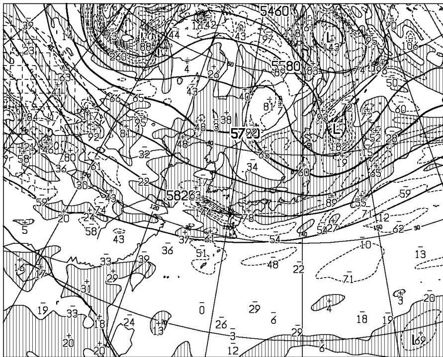
T=36 VALID 210000UTC HEIGHT (M), VORT (10** \times -6/SEC) AT 500hPa
