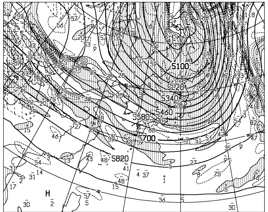
T=48 VALID 191200UTC HEIGHT (M), VORT (10**+6/SEC) AT 500hPa
