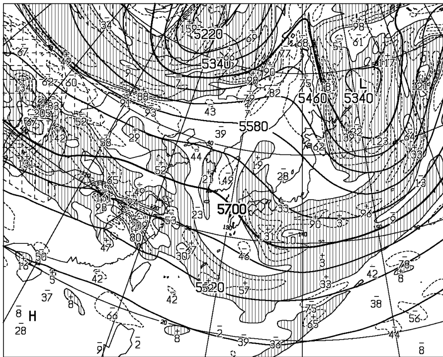
T=36 VALID 150000UTC HEIGHT (M), VORT (10 -6 /SEC) AT 500hPa
