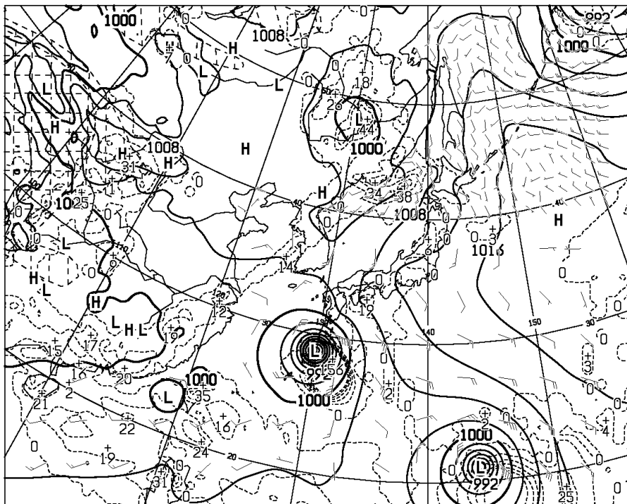
T=36 VALID 211200UTC SURFACE PRESS (hPa), PRECIP (MM) (24-36) WIND ARROW AT SURFACE
