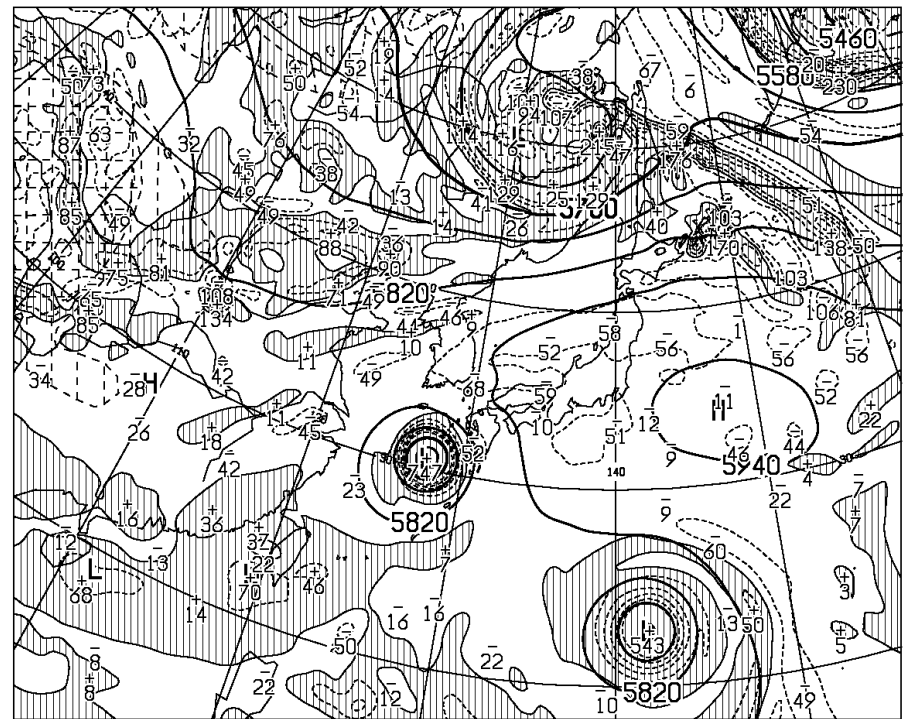
T=48 VALID 220000UTC HEIGHT (M), VORT (10** -6 /SEC) AT 500hPa
