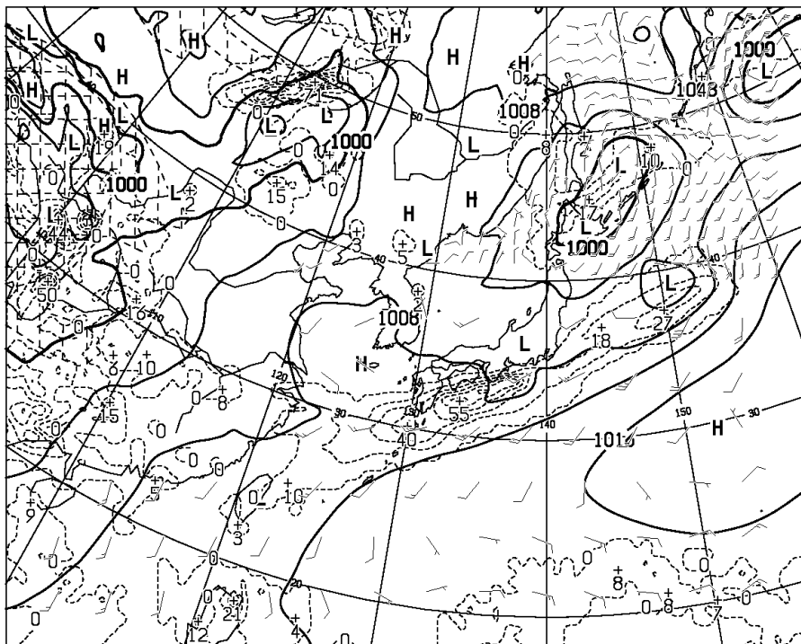
T=36 VALID 240000UTC SURFACE PRESS (hPa), PRECIP (MM) (24-36) WIND ARROW AT SURFACE
