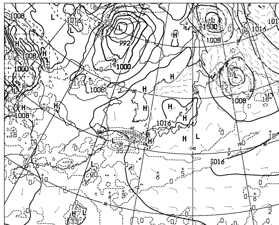
T=48 VALID 211200UTC SURFACE PRESS (hPa), PRECIP (MM) (36-48) WIND ARROW AT SURFACE
