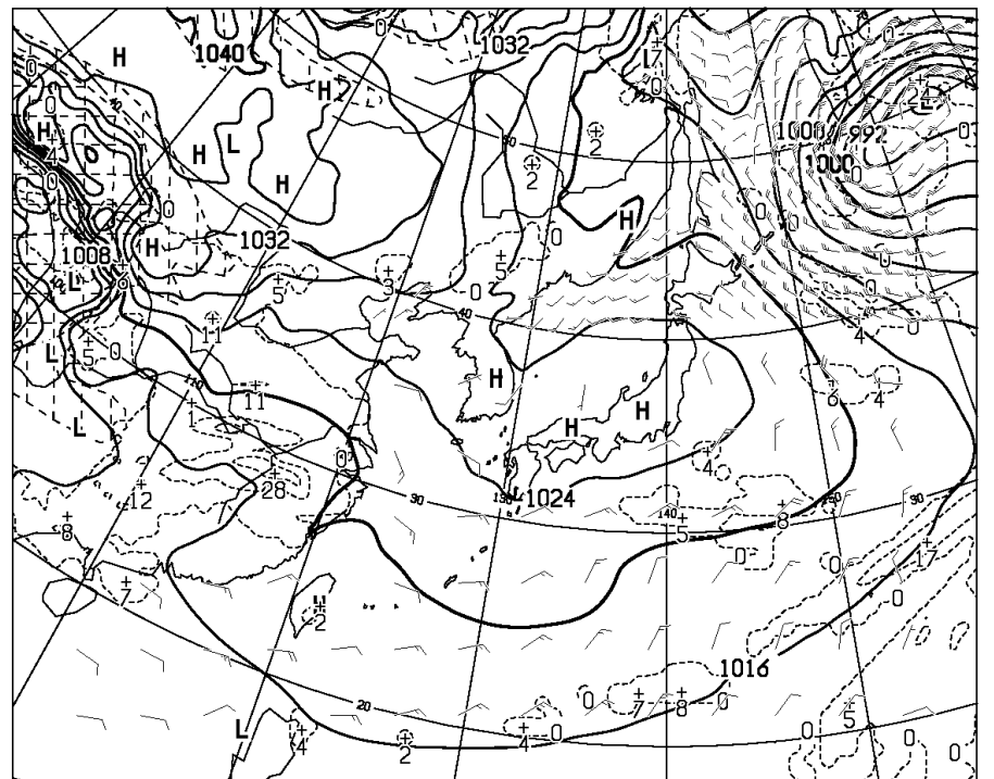
T=48 VALID 151200UTC SURFACE PRESS (hPa), PRECIP (MM) (36-48) WIND ARROW AT SURFACE
