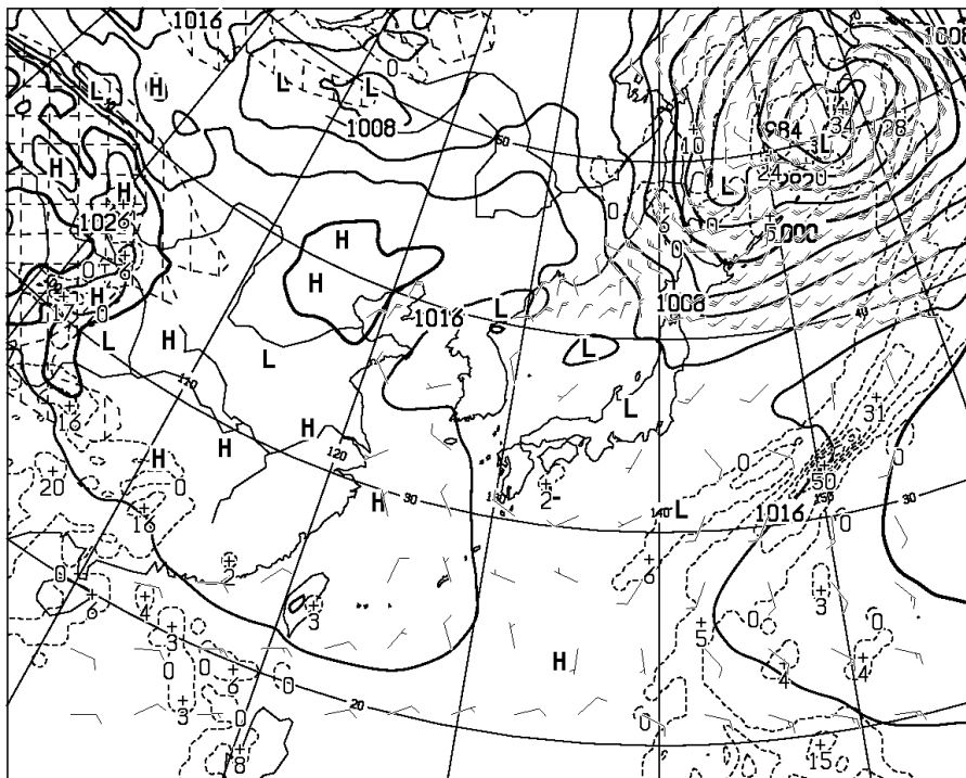
T=36 VALID 270000UTC SURFACE PRESS (hPa), PRECIP (MM) (24-36) WIND ARROW AT SURFACE
