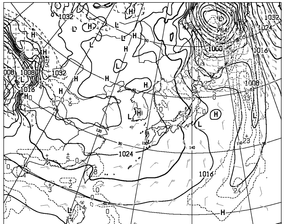
T=48 VALID 191200UTC SURFACE PRESS (hPa), PRECIP (MM) (36-48) WIND ARROW AT SURFACE
