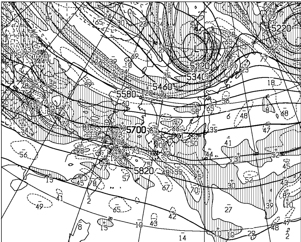
T=72 VALID 161200UTC HEIGHT (M), VORT (10**x-6/SEC) AT 500hPa
