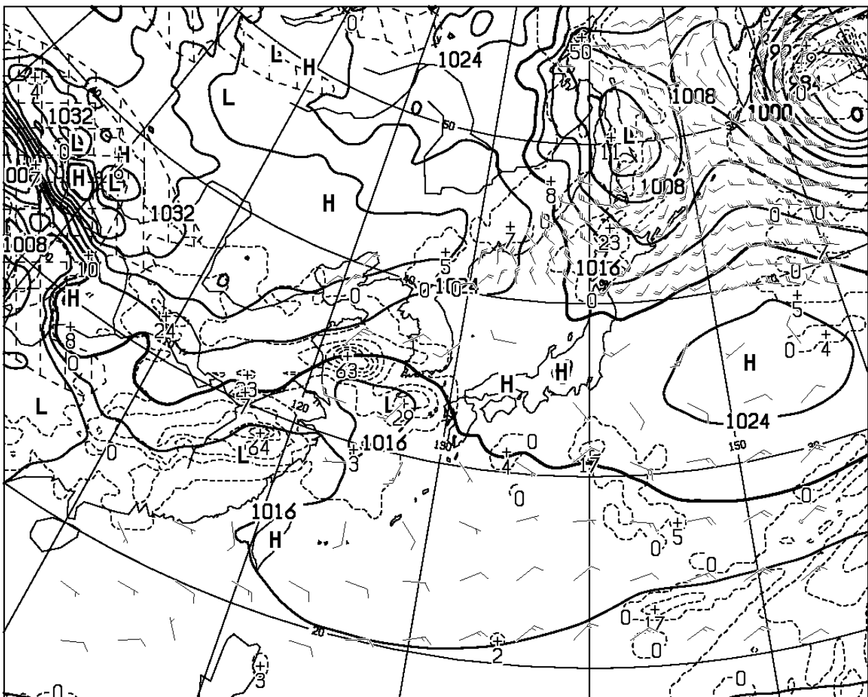
T=72 VALID 161200UTC SURFACE PRESS (hPa), PRECIP (MM) (48-72) WIND ARROW AT SURFACE
