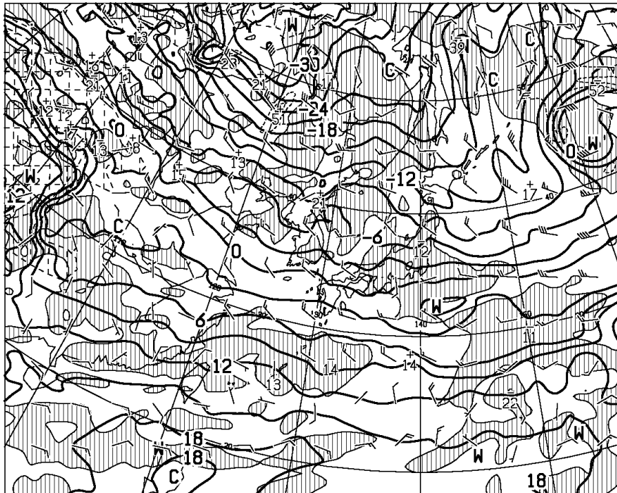
T=12 VALID 191200UTC TEMP (C), WIND ARROW AT 850hPa P-VEL (hPa/H) AT 700hPa
