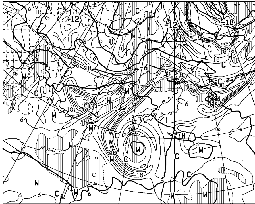
T=24 VALID 210000UTC TEMP (C) AT 500hPa T-TD (C) AT 700hPa
