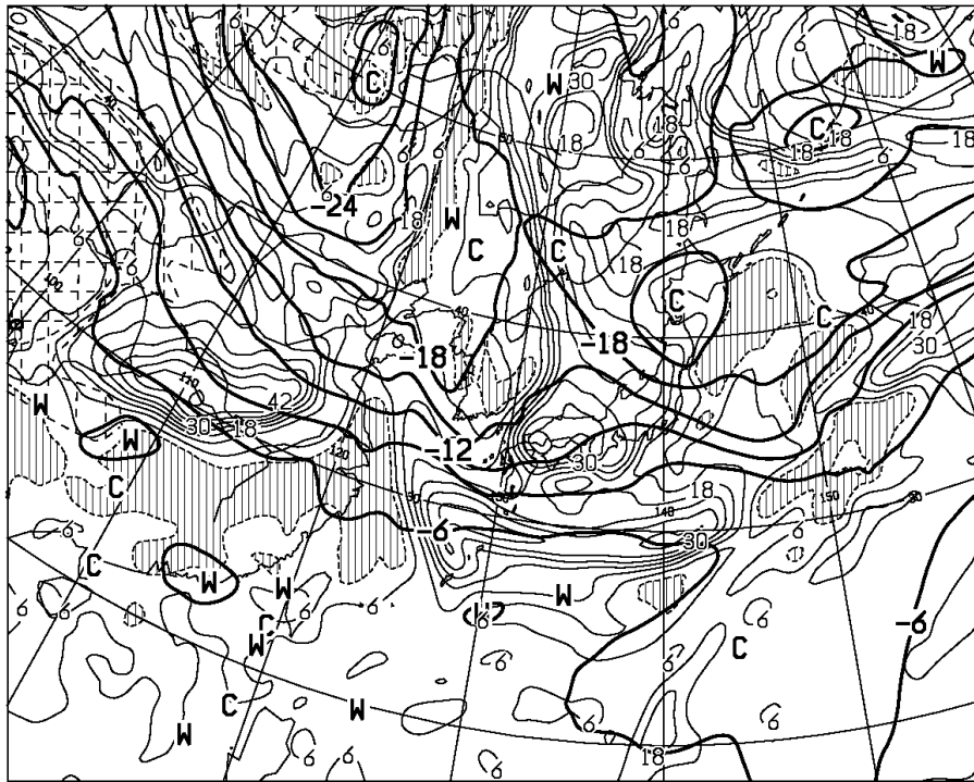
T=12 VALID 300000UTC TEMP (C) AT 500hPa T-TD (C) AT 700hPa
