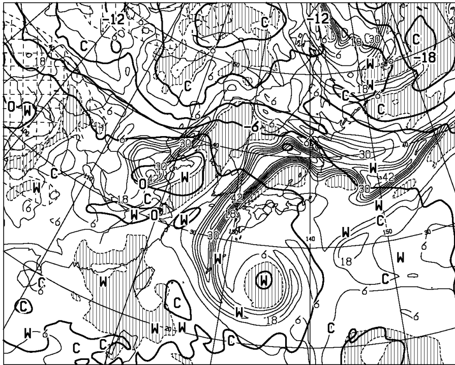
T=12 VALID 201200UTC TEMP (C) AT 500hPa T-TD (C) AT 700hPa
