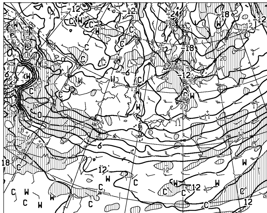
T=24 VALID 171200UTC TEMP (C), WIND ARROW AT 850hPa P-VEL (hPa/h) AT 700hPa
