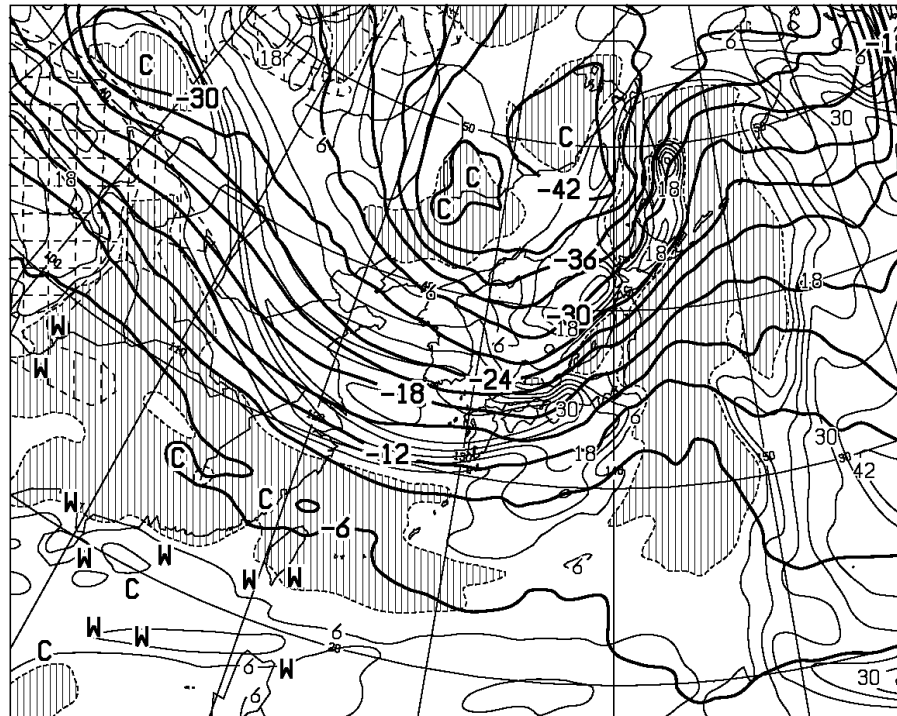
T=24 VALID 181200UTC TEMP (C) AT 500hPa T-TD (C) AT 700hPa
