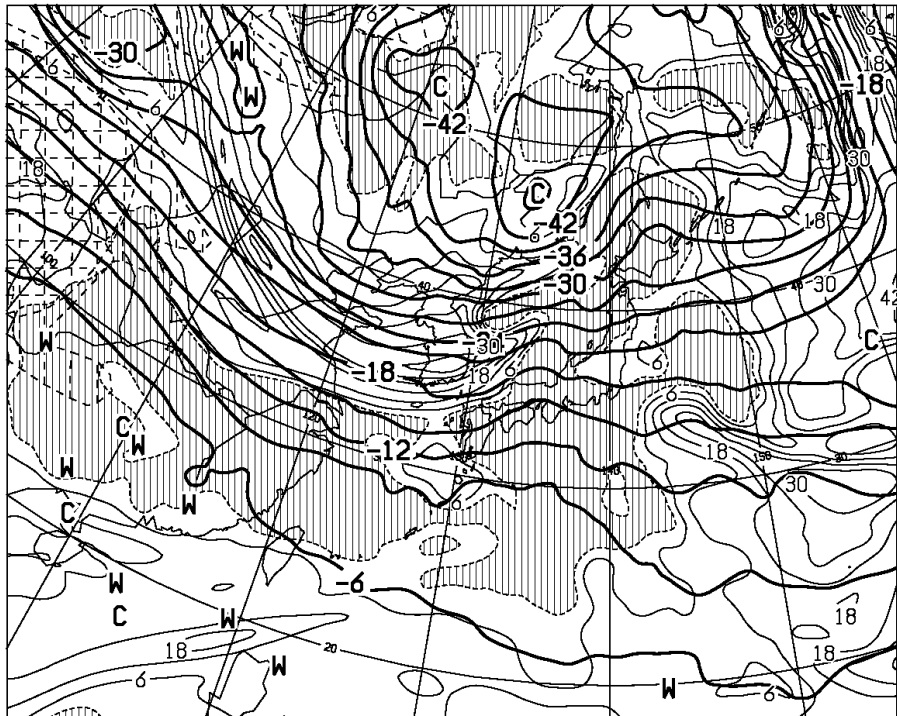
T=12 VALID 180000UTC TEMP (C) AT 500hPa T-TD (C) AT 700hPa
