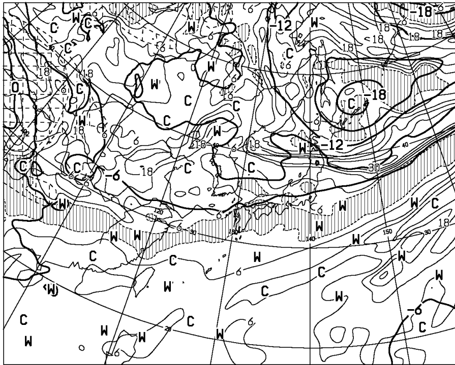
T=12 VALID 271200UTC TEMP (C) AT 500hPa T-TD (C) AT 700hPa
