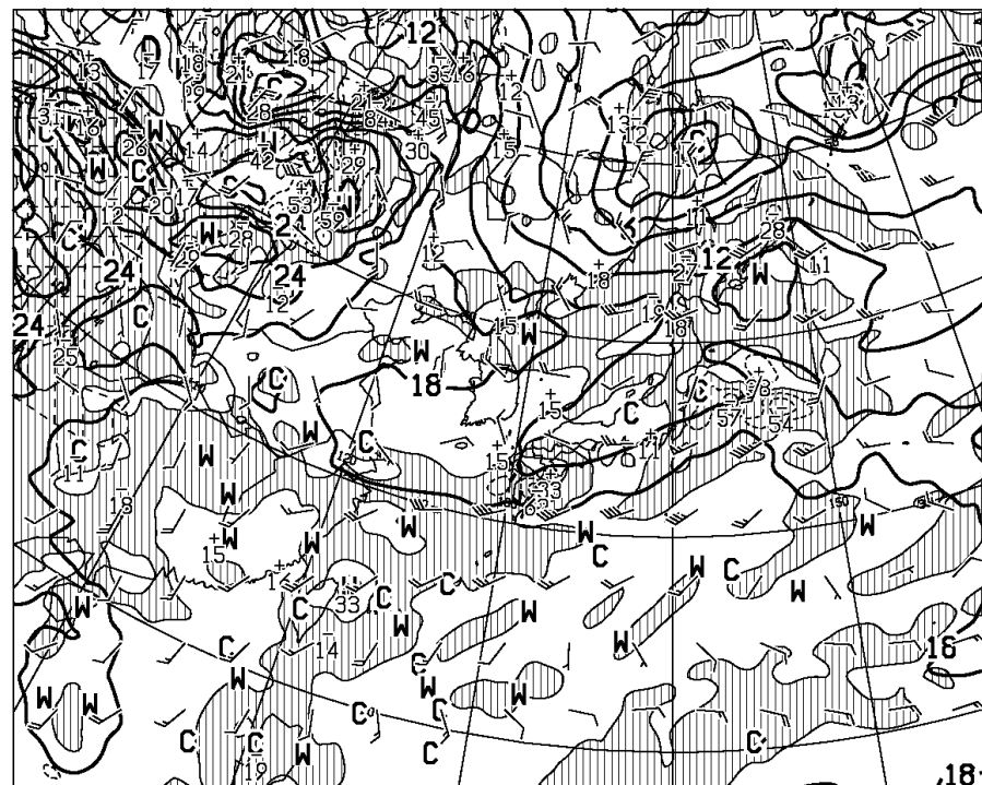
T=24 VALID 231200UTC TEMP (C), WIND ARROW AT 850hPa P-VEL (hPa/H) AT 700hPa
