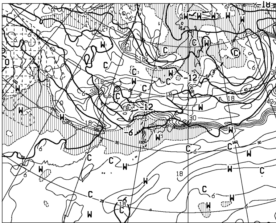
T=12 VALID 230000UTC TEMP (C) AT 500hPa T-TD (C) AT 700hPa
