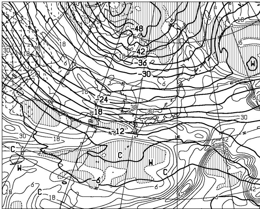
T=12 VALID 191200UTC TEMP (C) AT 500hPa T-TD (C) AT 700hPa
