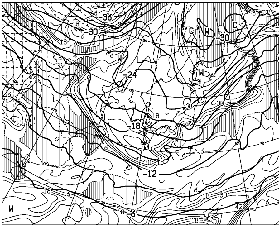
T=12 VALID 140000UTC TEMP (C) AT 500hPa T-TD (C) AT 700hPa
