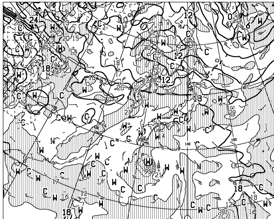
T=24 VALID 210000UTC TEMP (C), WIND ARROW AT 850hPa P-VEL (hPa/h) AT 700hPa
