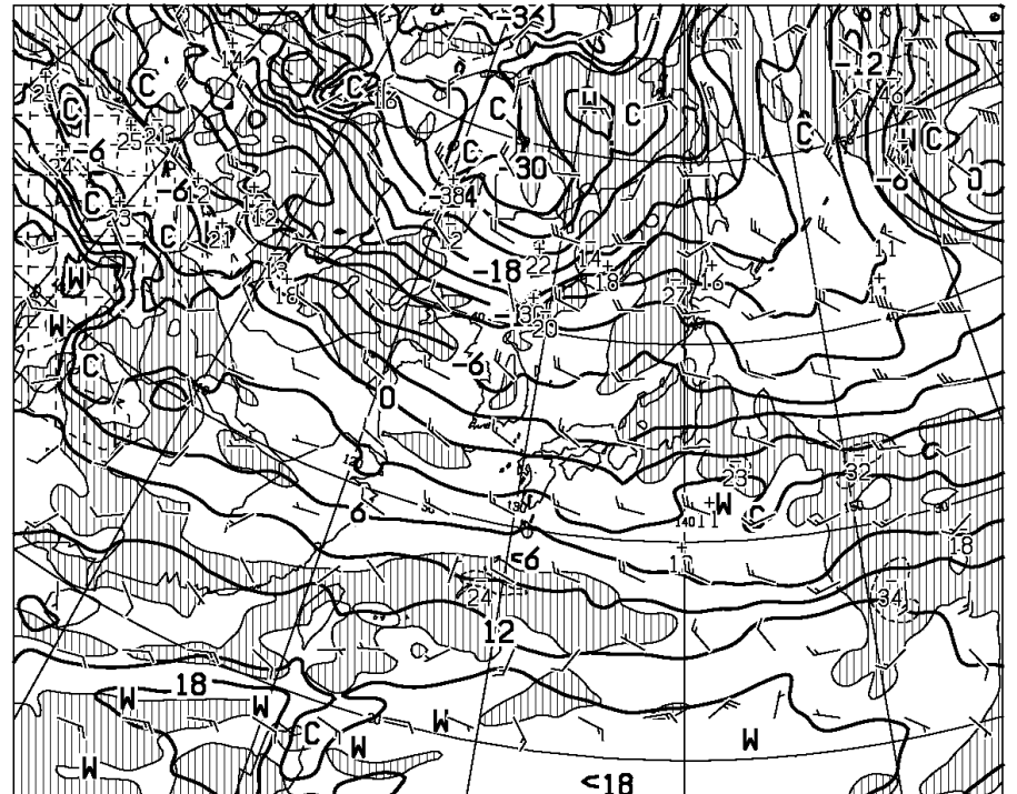
T=24 VALID 200000UTC TEMP (C), WIND ARROW AT 850hPa P-VEL (hPa/H) AT 700hPa
