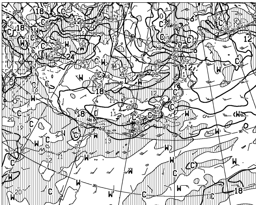
T=12 VALID 230000UTC TEMP (C), WIND ARROW AT 850hPa P-VEL (hPa/H) AT 700hPa
