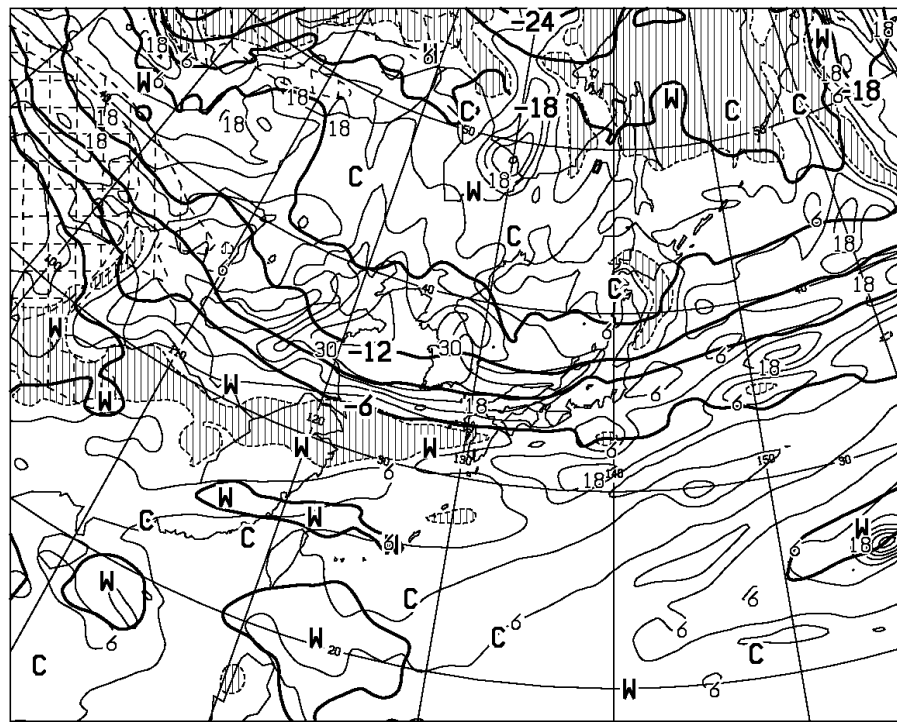
T=24 VALID 201200UTC TEMP (C) AT 500hPa T-TD (C) AT 700hPa
