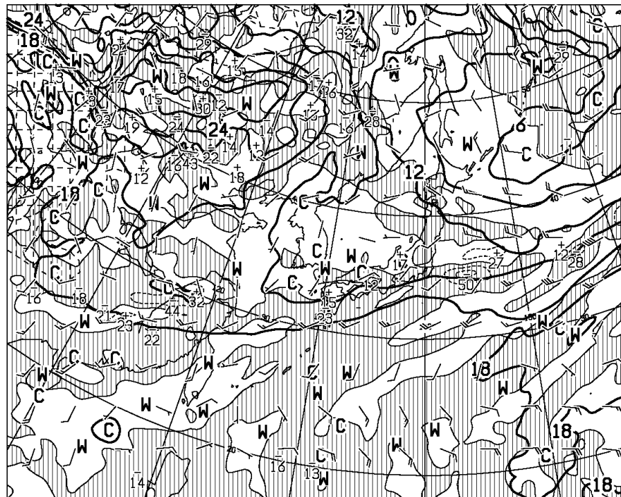
T=24 VALID 280000UTC TEMP (C), WIND ARROW AT 850hPa P-VEL (hPa/H) AT 700hPa
