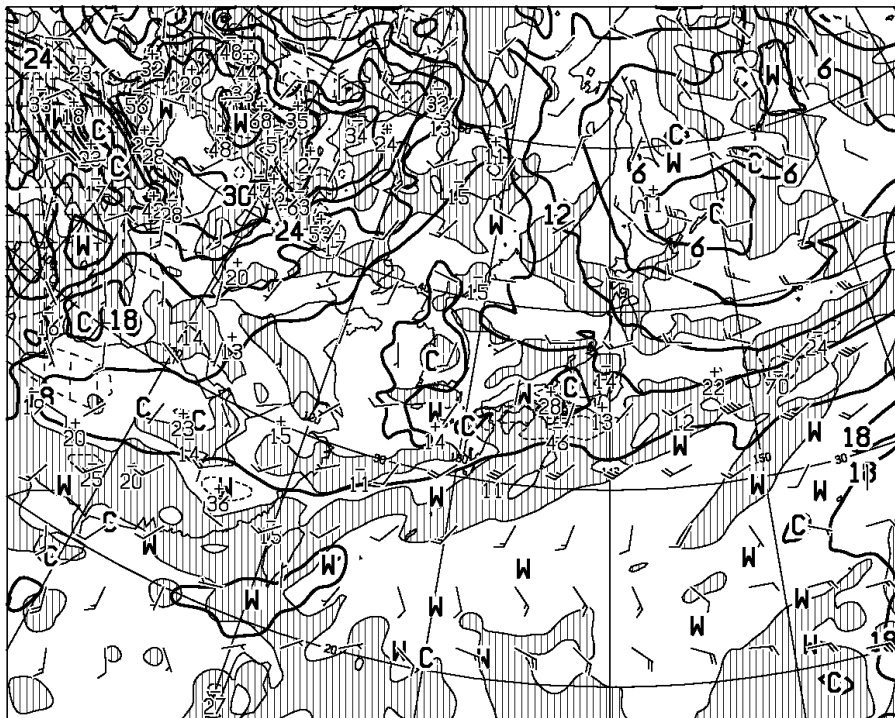
T=12 VALID 271200UTC TEMP (C), WIND ARROW AT 850hPa P-VEL (hPa/H) AT 700hPa
