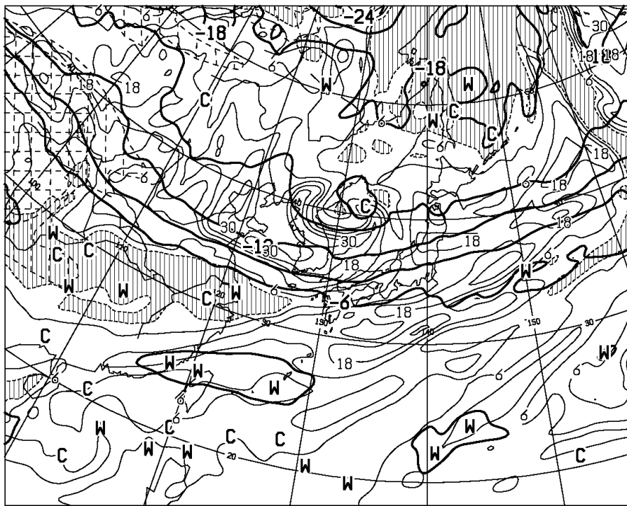
T=12 VALID 200000UTC TEMP (C) AT 500hPa T-TD (C) AT 700hPa
