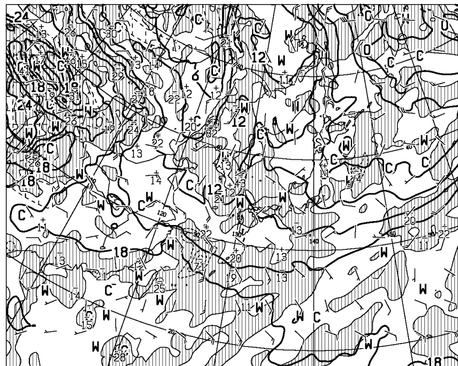
T=24 VALID 301200UTC TEMP (C), WIND ARROW AT 850hPa P-VEL (hPa/h) AT 700hPa
