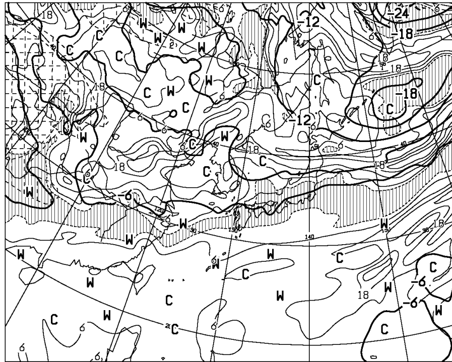
T=24 VALID 280000UTC TEMP (C) AT 500hPa T-TD (C) AT 700hPa
