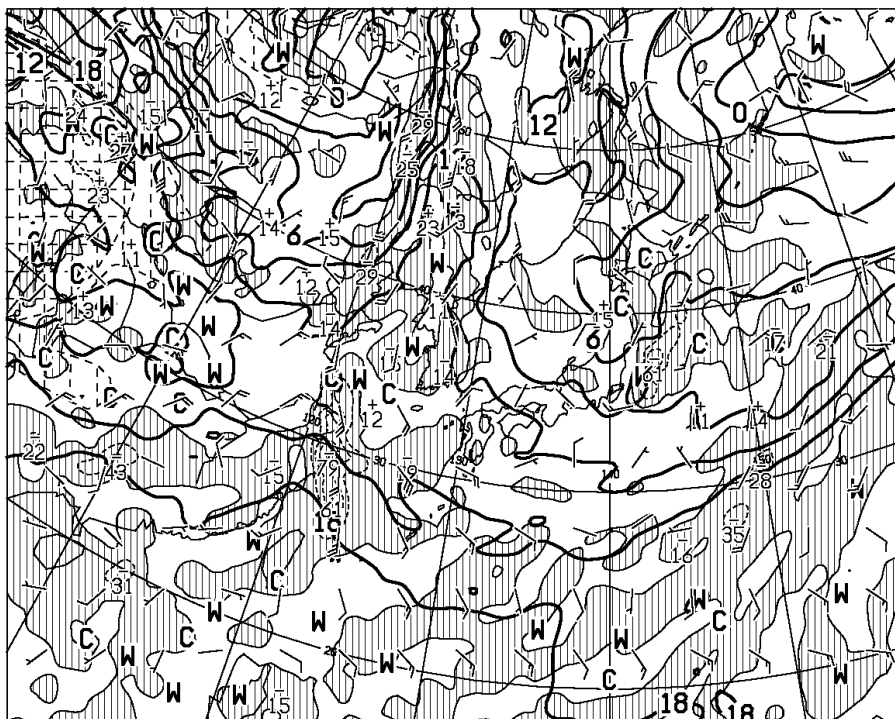
T=12 VALID 300000UTC TEMP (C), WIND ARROW AT 850hPa P-VEL (hPa/h) AT 700hPa
