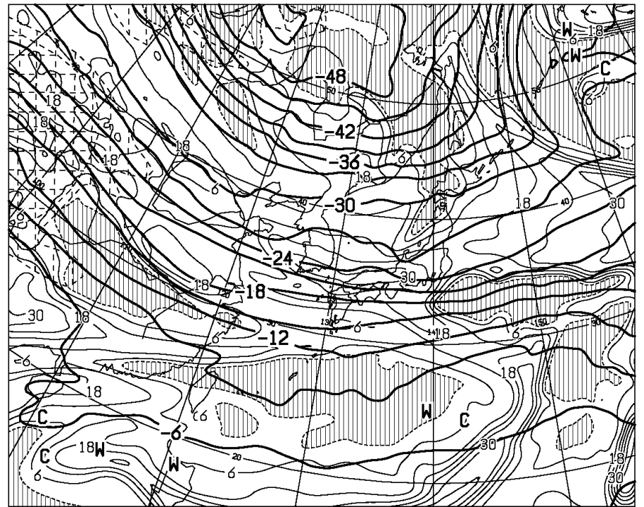
T=24 VALID 200000UTC TEMP (C) AT 500hPa T-TD (C) AT 700hPa
