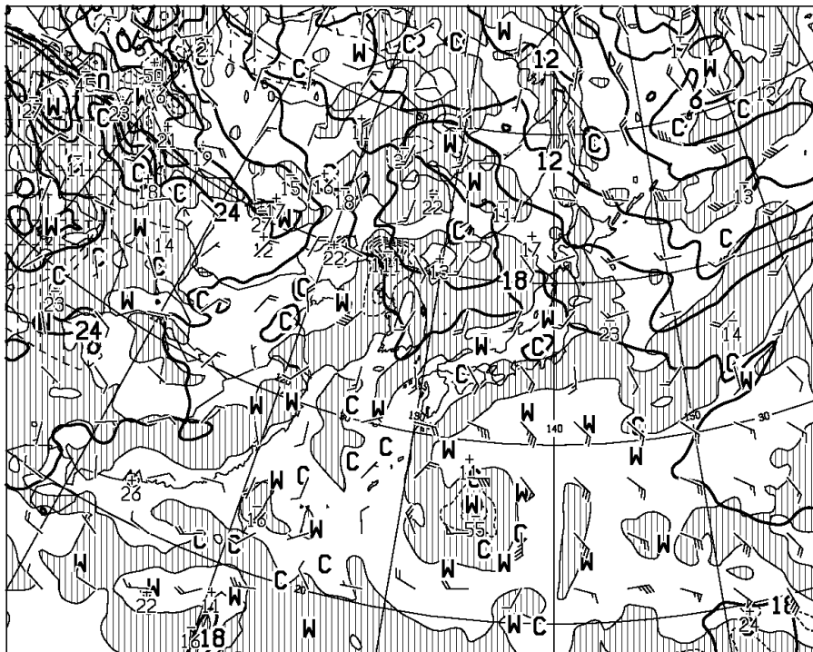
T=12 VALID 201200UTC TEMP (C), WIND ARROW AT 850hPa P-VEL (hPa/h) AT 700hPa
