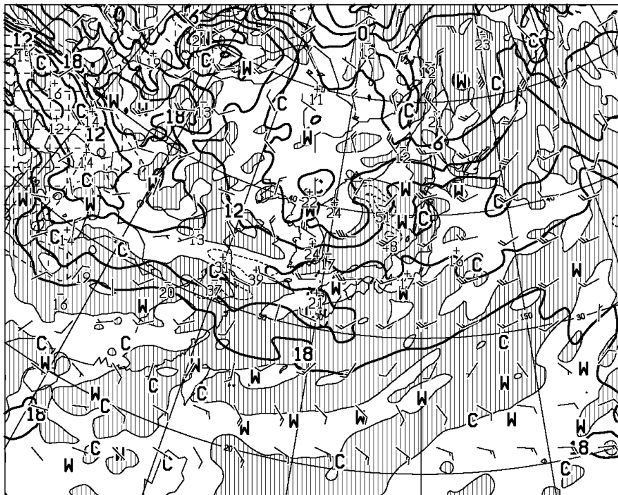
T=12 VALID 200000UTC TEMP (C), WIND ARROW AT 850hPa P-VEL (hPa/H) AT 700hPa
