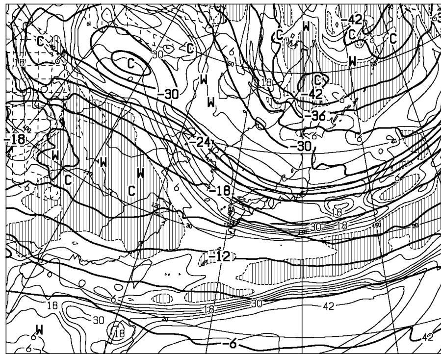
T=24 VALID 171200UTC TEMP (C) AT 500hPa T-TD (C) AT 700hPa
