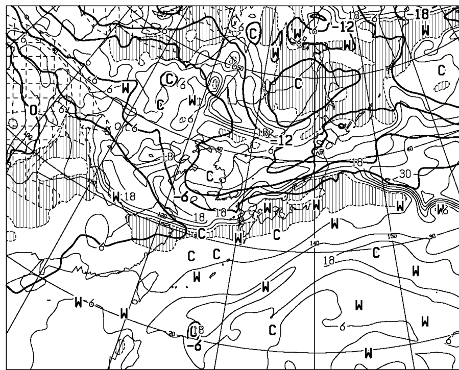
T=24 VALID 231200UTC TEMP (C) AT 500hPa T-TD (C) AT 700hPa
