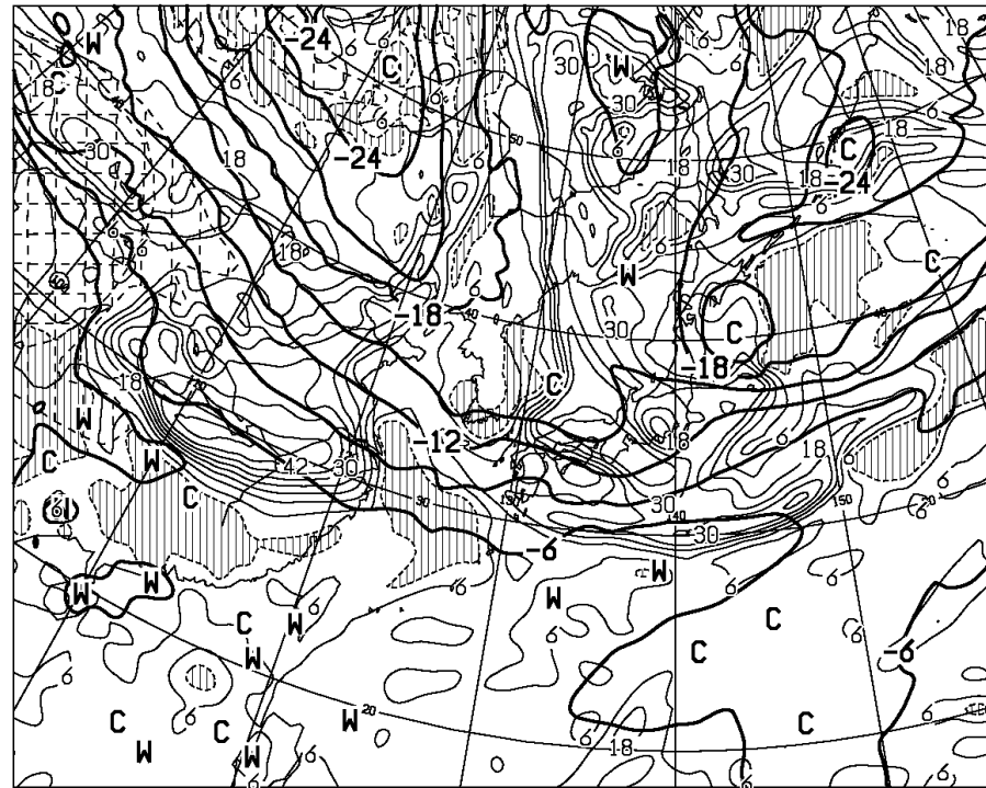
T=24 VALID 301200UTC TEMP (C) AT 500hPa T-TD (C) AT 700hPa
