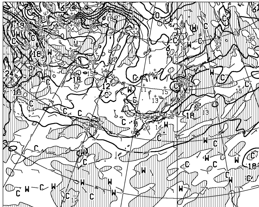
T=24 VALID 201200UTC TEMP (C), WIND ARROW AT 850hPa P-VEL (hPa/H) AT 700hPa
