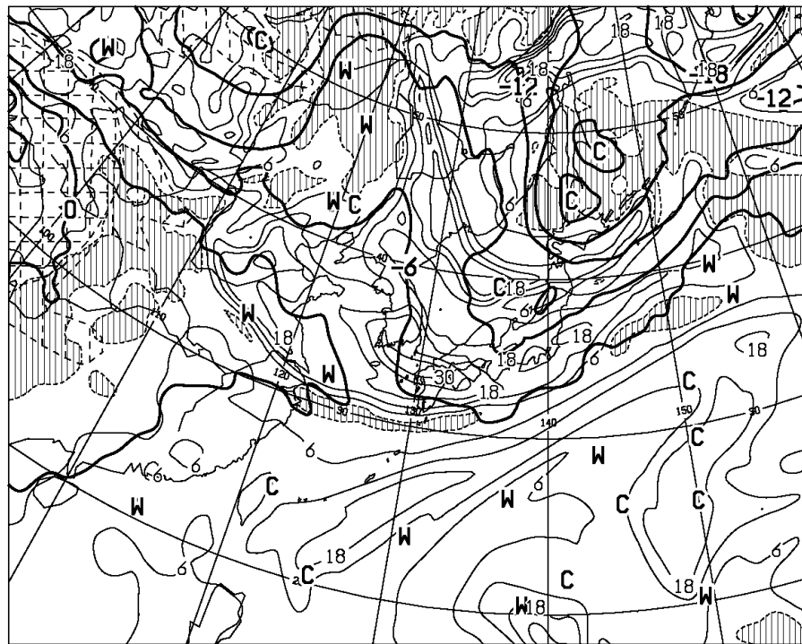
T=48 VALID 241200UTC TEMP (C) AT 500hPa T-TD (C) AT 700hPa
