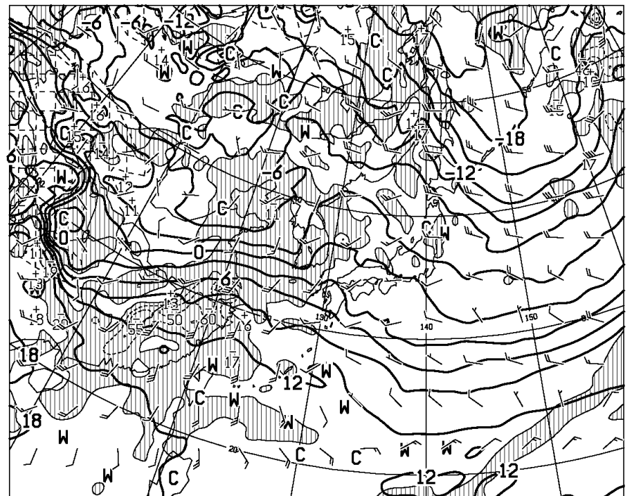
T=48 VALID 181200UTC TEMP (C), WIND ARROW AT 850hPa P-VEL (hPa/h) AT 700hPa
