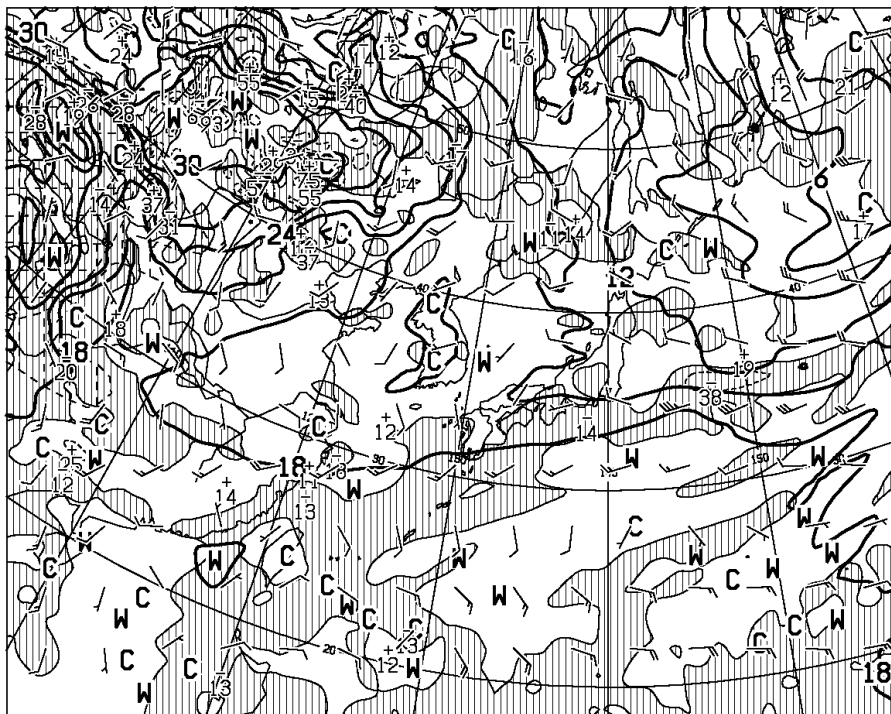
T=36 VALID 281200UTC TEMP (C), WIND ARROW AT 850hPa P-VEL (hPa/H) AT 700hPa
