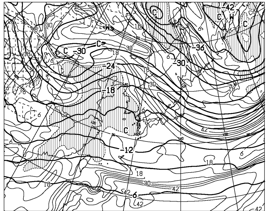
T=48 VALID 181200UTC TEMP (C) AT 500hPa T-TD (C) AT 700hPa
