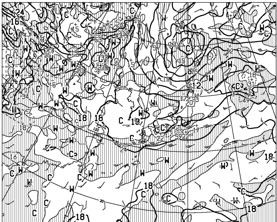
T=36 VALID 240000UTC TEMP (C), WIND ARROW AT 850hPa P-VEL (hPa/h) AT 700hPa
