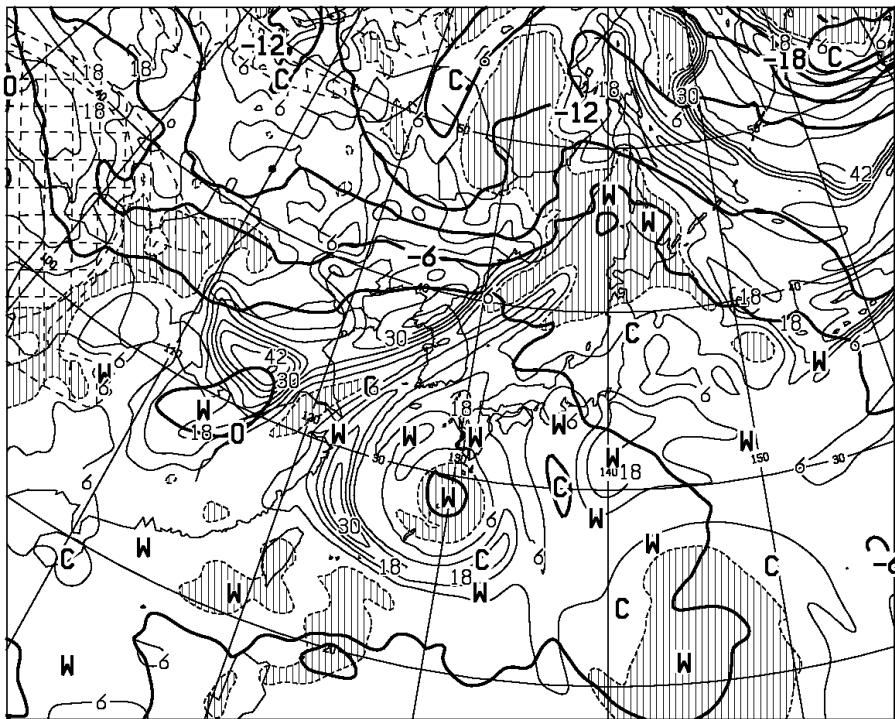
T=36 VALID 211200UTC TEMP (C) AT 500hPa T-TD (C) AT 700hPa
