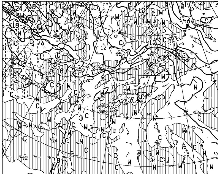
T=48 VALID 220000UTC TEMP (C), WIND ARROW AT 850hPa P-VEL (hPa/h) AT 700hPa
