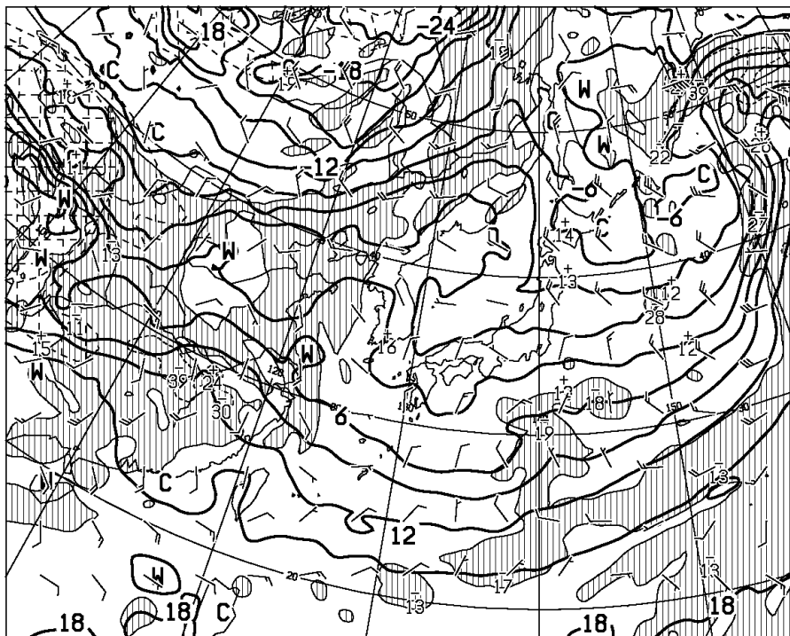
T=36 VALID 150000UTC TEMP (C), WIND ARROW AT 850hPa P-VEL (hPa/h) AT 700hPa
