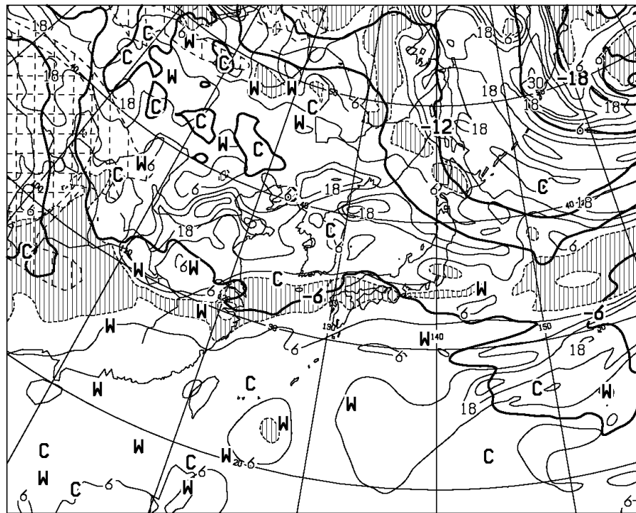
T=48 VALID 290000UTC TEMP (C) AT 500hPa T-TD (C) AT 700hPa
