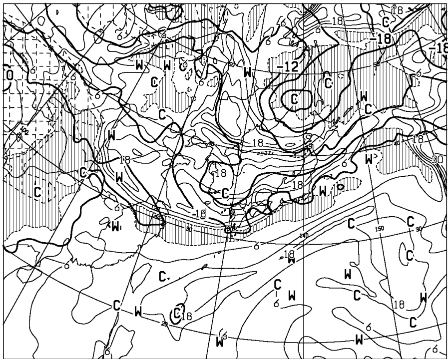
T=36 VALID 240000UTC TEMP (C) AT 500hPa T-TD (C) AT 700hPa
