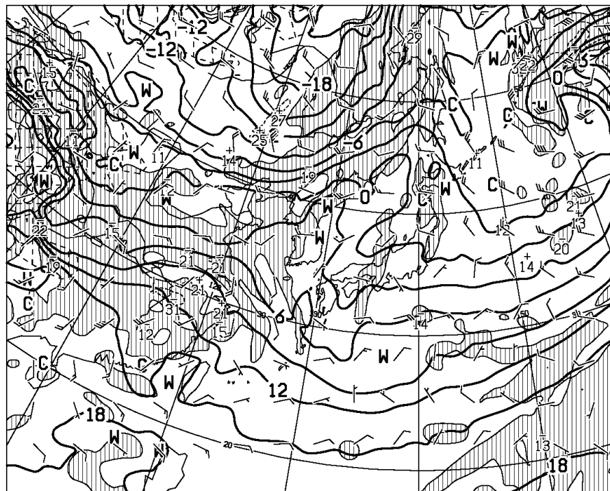
T=48 VALID 151200UTC TEMP (C), WIND ARROW AT 850hPa P-VEL (hPa/h) AT 700hPa
