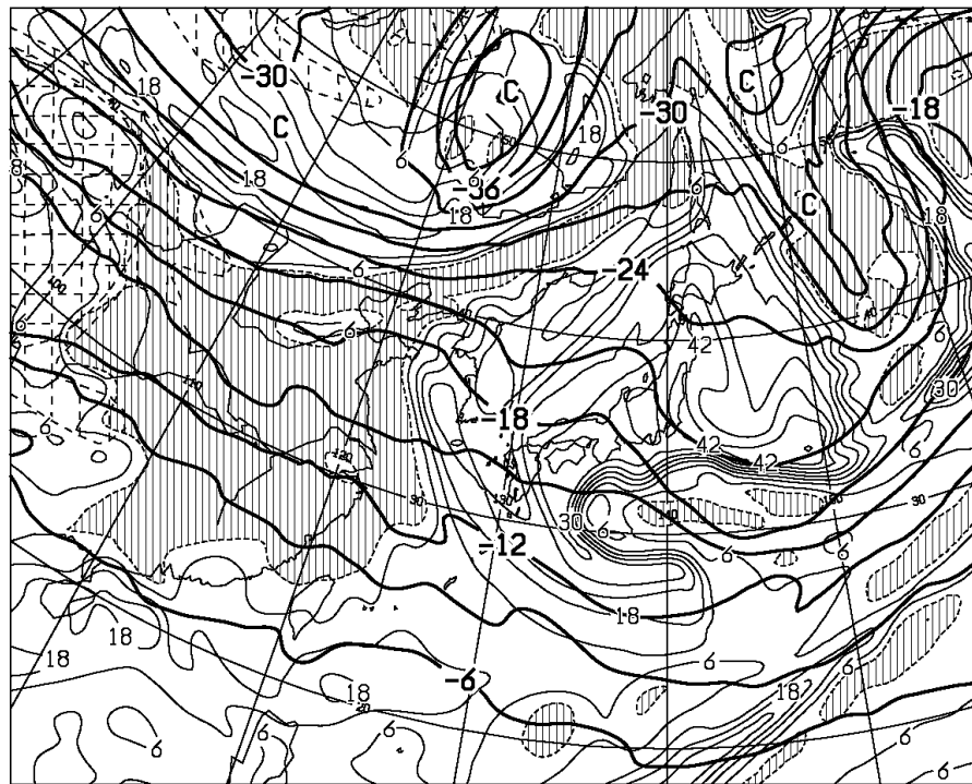
T=48 VALID 151200UTC TEMP (C) AT 500hPa T-TD (C) AT 700hPa
