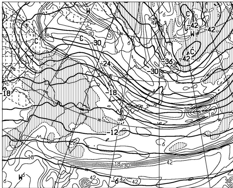
T=36 VALID 180000UTC TEMP (C) AT 500hPa T-TD (C) AT 700hPa
