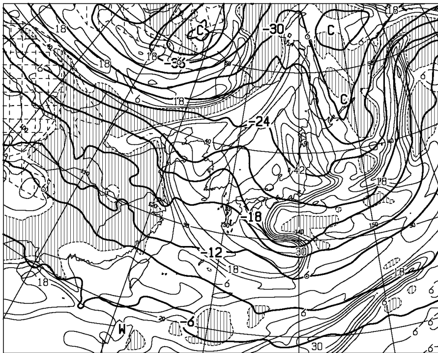
T=36 VALID 150000UTC TEMP (C) AT 500hPa T-TD (C) AT 700hPa
