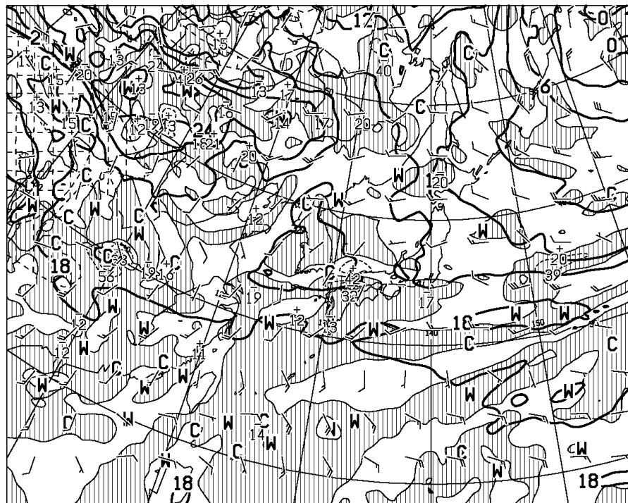
T=48 VALID 290000UTC TEMP (C), WIND ARROW AT 850hPa P-VEL (hPa/H) AT 700hPa
