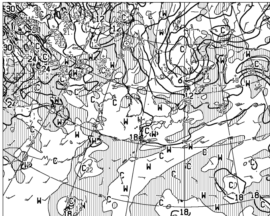
T=48 VALID 241200UTC TEMP (C), WIND ARROW AT 850hPa P-VEL (hPa/h) AT 700hPa
