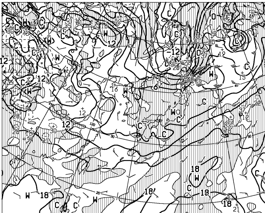
T=36 VALID 270000UTC TEMP (C), WIND ARROW AT 850hPa P-VEL (hPa/h) AT 700hPa
