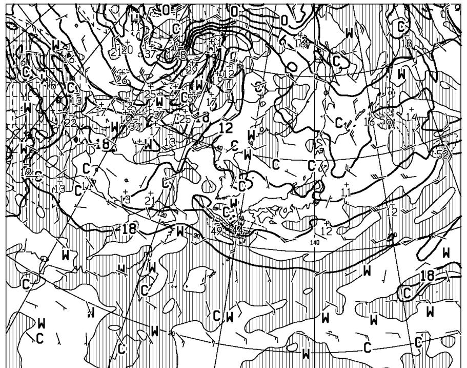
T=48 VALID 211200UTC TEMP (C), WIND ARROW AT 850hPa P-VEL (hPa/H) AT 700hPa
