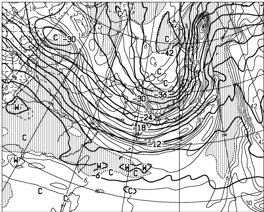
T=36 VALID 190000UTC TEMP (C) AT 500hPa T-D (C) AT 700hPa
