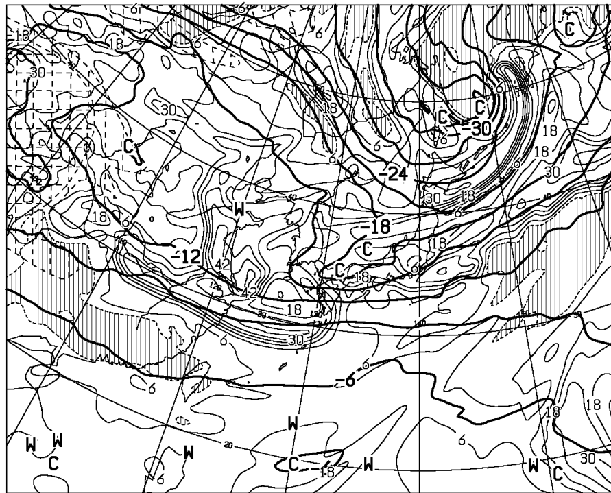
T=48 VALID 271200UTC TEMP (C) AT 500hPa T-TD (C) AT 700hPa
