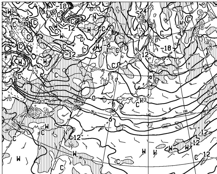
T=36 VALID 180000UTC TEMP (C), WIND ARROW AT 850hPa P-VEL (hPa/h) AT 700hPa
