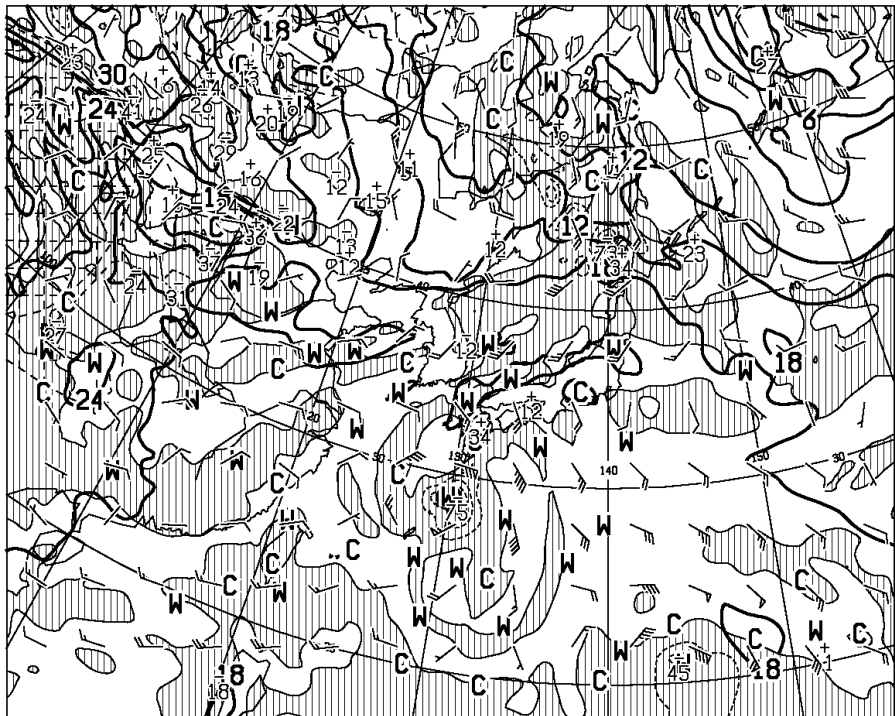
T=36 VALID 211200UTC TEMP (C), WIND ARROW AT 850hPa P-VEL (hPa/h) AT 700hPa
