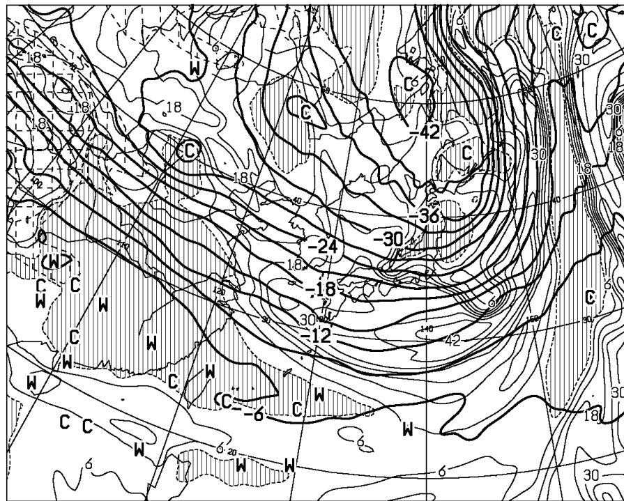
T=48 VALID 191200UTC TEMP (C) AT 500hPa T-D (C) AT 700hPa
