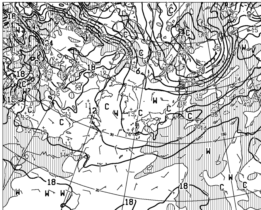
T=48 VALID 271200UTC TEMP (C), WIND ARROW AT 850hPa P-VEL (hPa/h) AT 700hPa
