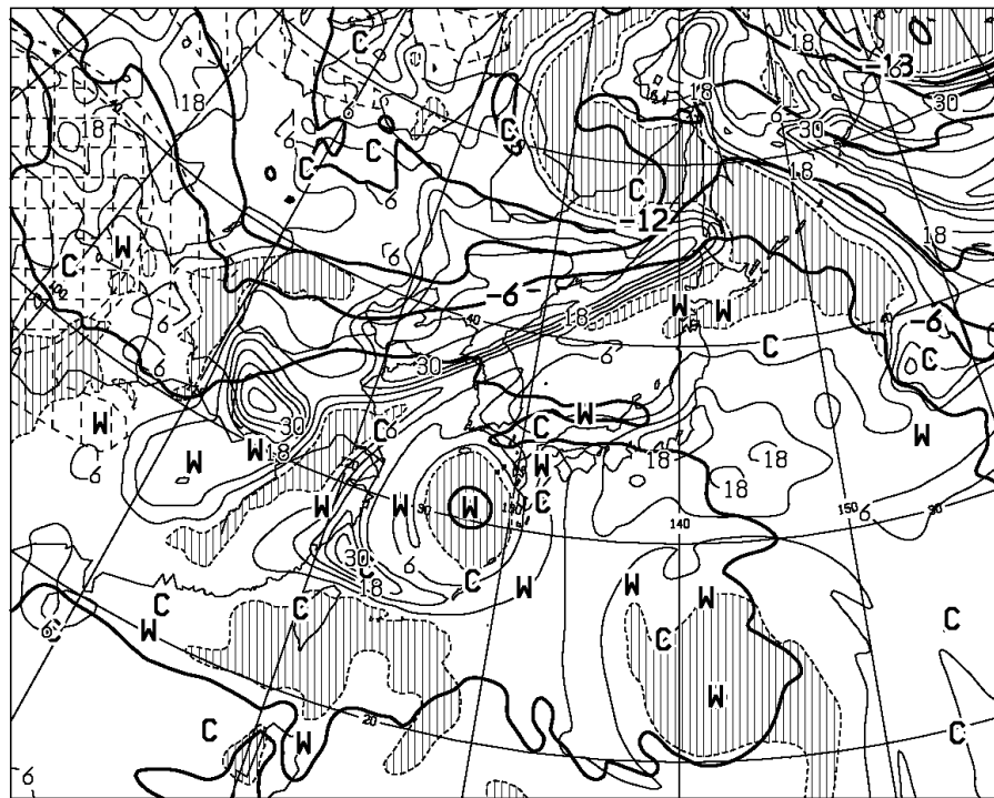
T=48 VALID 220000UTC TEMP (C) AT 500hPa T-TD (C) AT 700hPa
