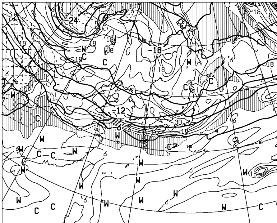
T=36 VALID 210000UTC TEMP (C) AT 500hPa T-TD (C) AT 700hPa
