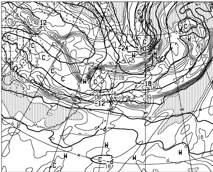
T=36 VALID 270000UTC TEMP (C) AT 500hPa T-TD (C) AT 700hPa
