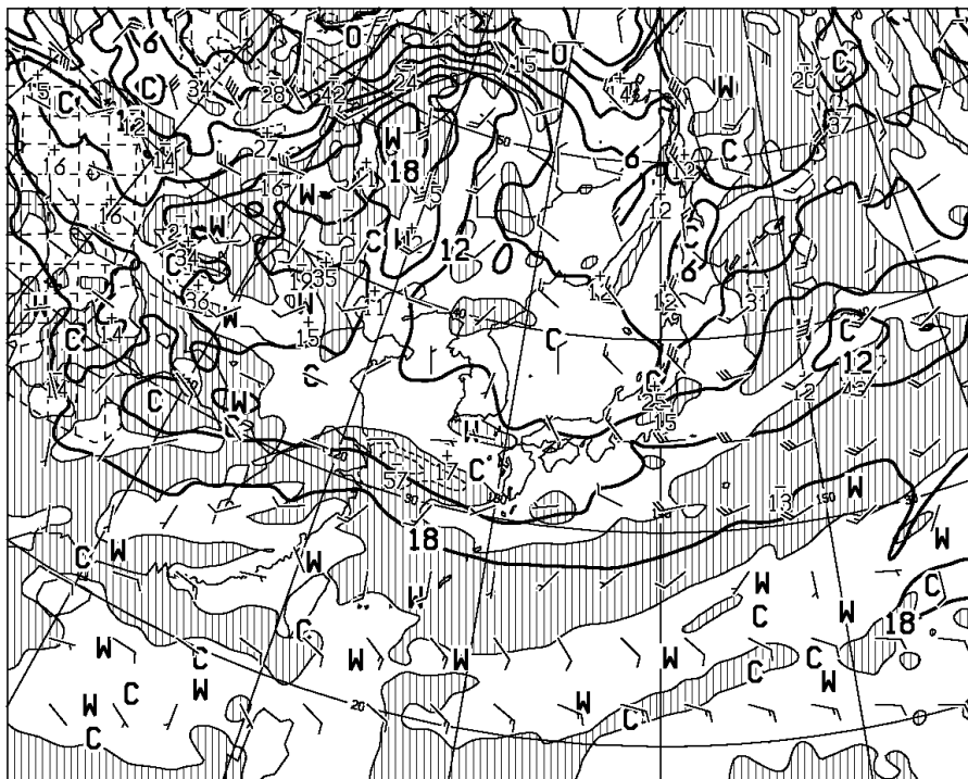
T=36 VALID 210000UTC TEMP (C), WIND ARROW AT 850hPa P-VEL (hPa/H) AT 700hPa
