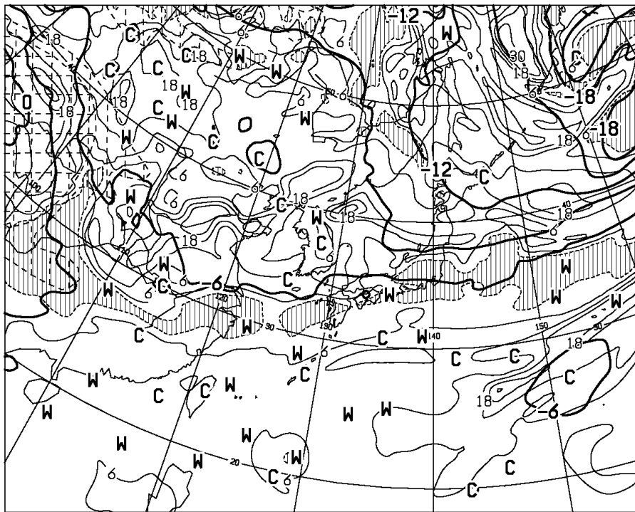
T=36 VALID 281200UTC TEMP (C) AT 500hPa T-TD (C) AT 700hPa
