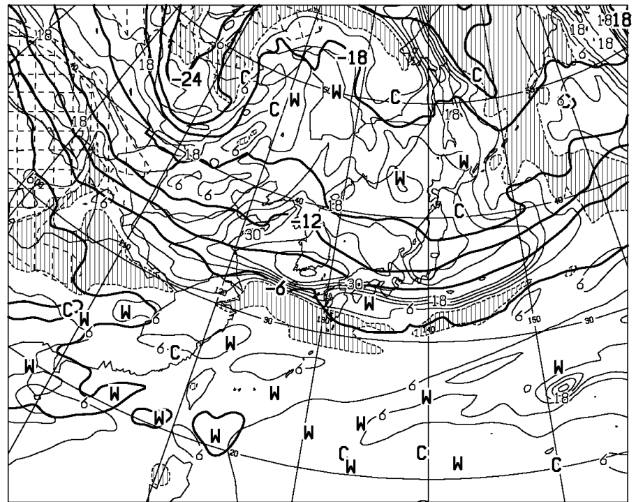
T=48 VALID 211200UTC TEMP (C) AT 500hPa T-TD (C) AT 700hPa
