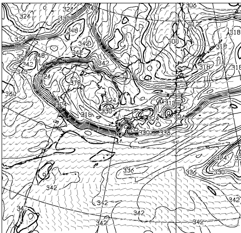
T=48 850hPa: E.P.TEMP(K),WIND(KNOTS) VALID 241200UTC
