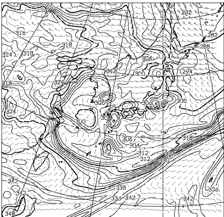
T=48 850hPa: E.P.TEMP(K),WIND(KNOTS) VALID 281200UTC
