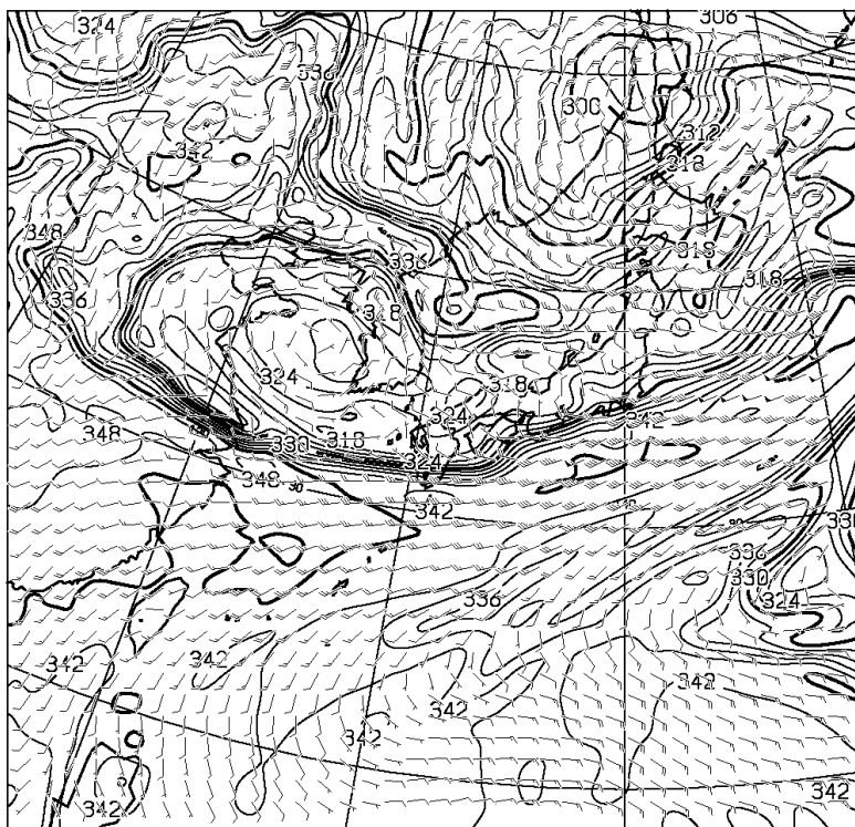
T=36 850hPa: E.P.TEMP(K),WIND(KNOTS) VALID 240000UTC
