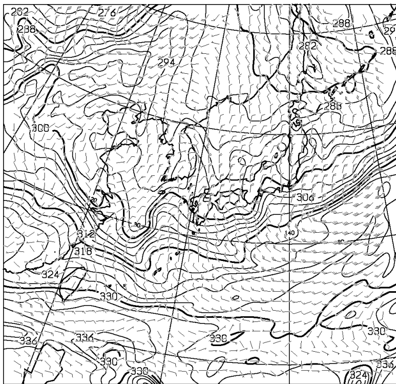
T=12 850hPa: E.P. TEMP(K), WIND(KNOTS) VALID 140000UTC
