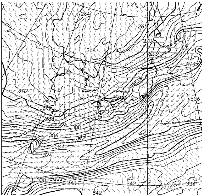
T=48 850hPa: E.P.TEMP(K),WIND(KNOTS) VALID 161200UTC
