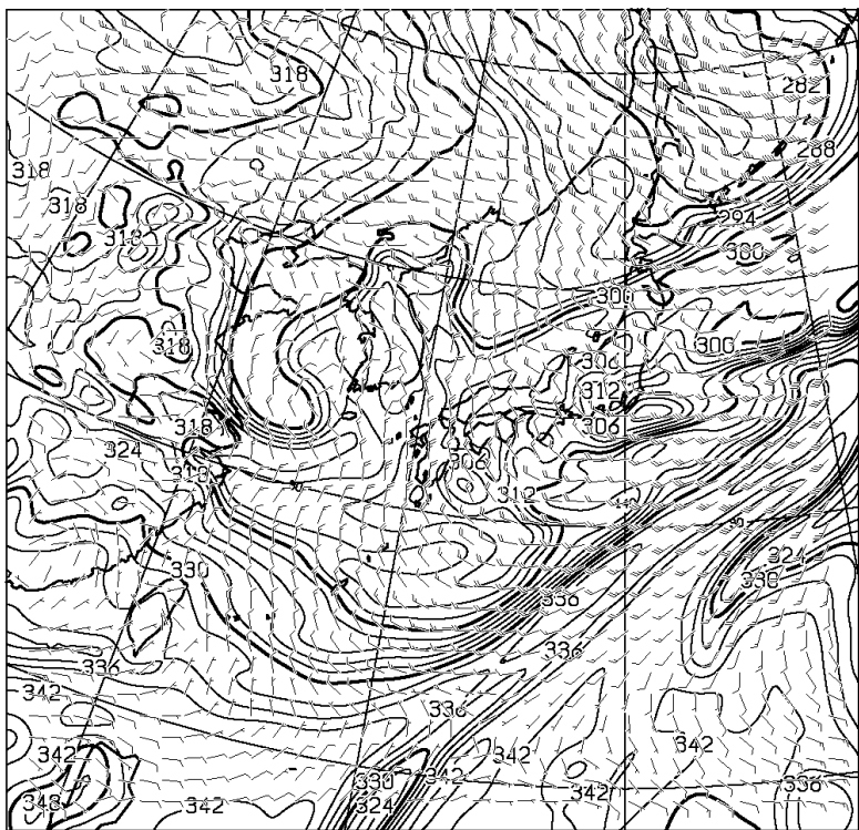
T=24 850hPa: E.P.TEMP(K),WIND(KNOTS) VALID 271200UTC
