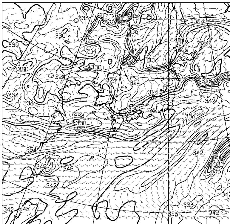
T=12 850hPa: E.P. TEMP(K), WIND(KNOTS) VALID 251200UTC
