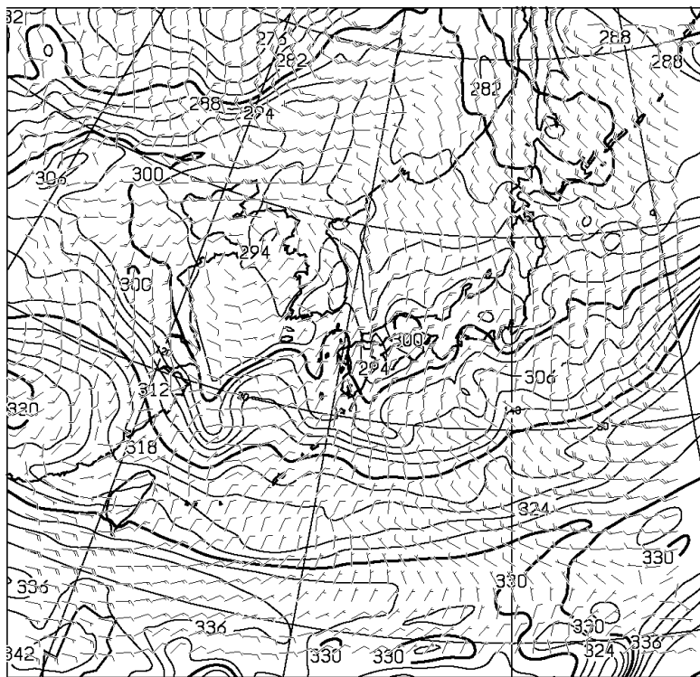
T=24 850hPa: E.P. TEMP(K), WIND(KNOTS) VALID 141200UTC
