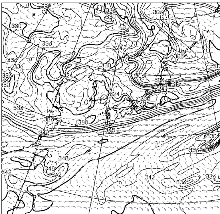
T=48 850hPa: E.P. TEMP(K), WIND(KNOTS) VALID 270000UTC
