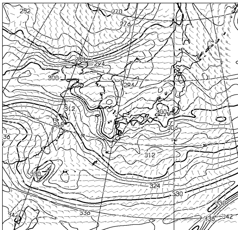
T=48 850hPa: E.P. TEMP(K), WIND(KNOTS) VALID 151200UTC
