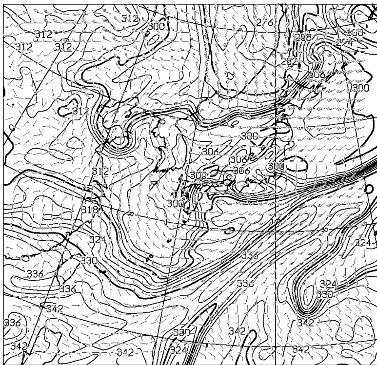
T=12 850hPa: E.P.TEMP(K),WIND(KNOTS) VALID 270000UTC
