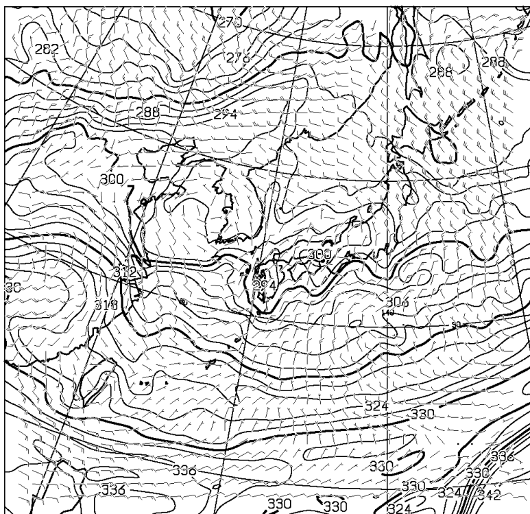
T=36 850hPa: E.P. TEMP(K), WIND(KNOTS) VALID 150000UTC
