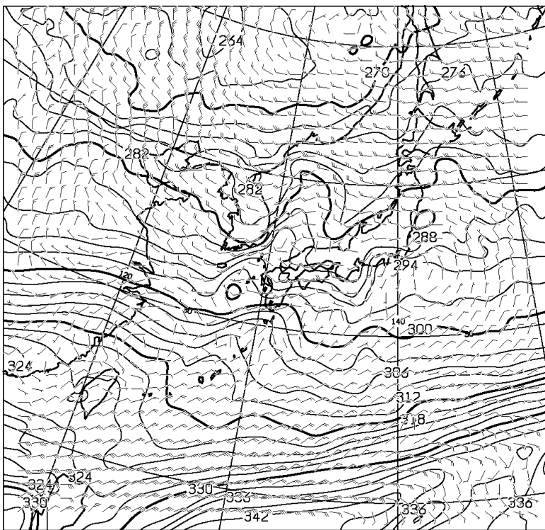
T=12 850hPa: E.P.TEMP(K),WIND(KNOTS) VALID 150000UTC
