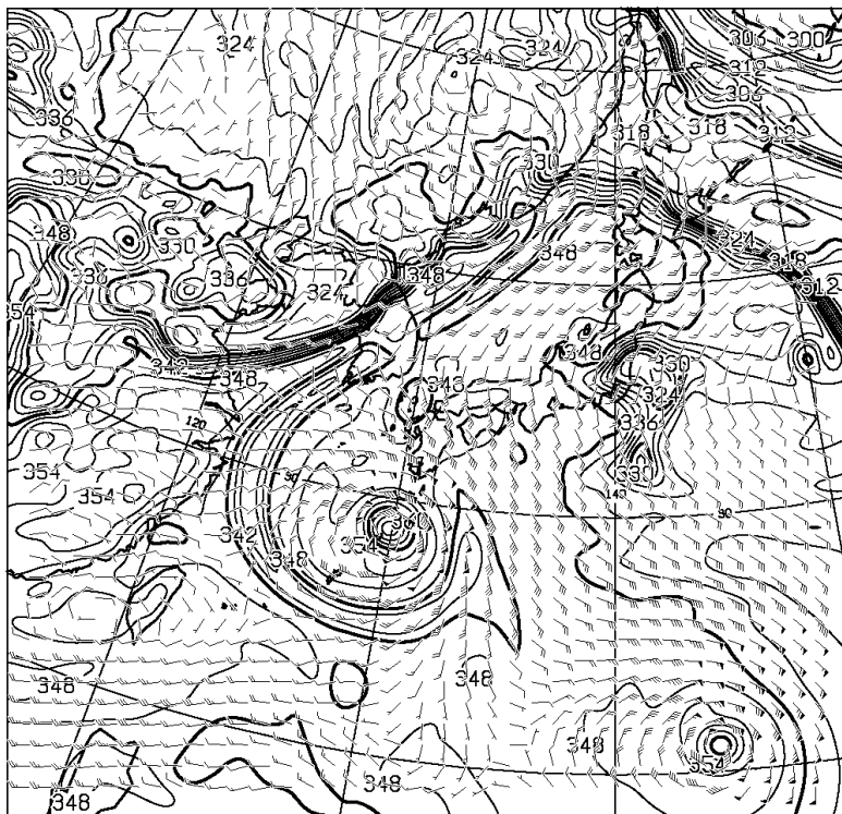
T=36 850hPa: E.P.TEMP(K),WIND(KNOTS) VALID 211200UTC
