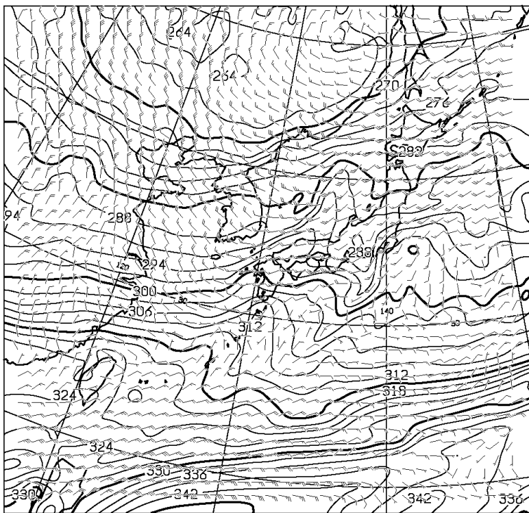
T=24 850hPa: E.P.TEMP(K),WIND(KNOTS) VALID 151200UTC
