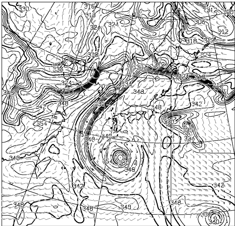
T=24 850hPa: E.P.TEMP(K),WIND(KNOTS) VALID 210000UTC
