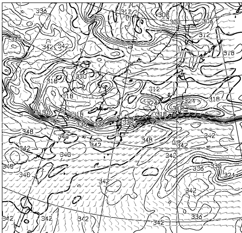
T=12 850hPa: E.P.TEMP(K),WIND(KNOTS) VALID 230000UTC
