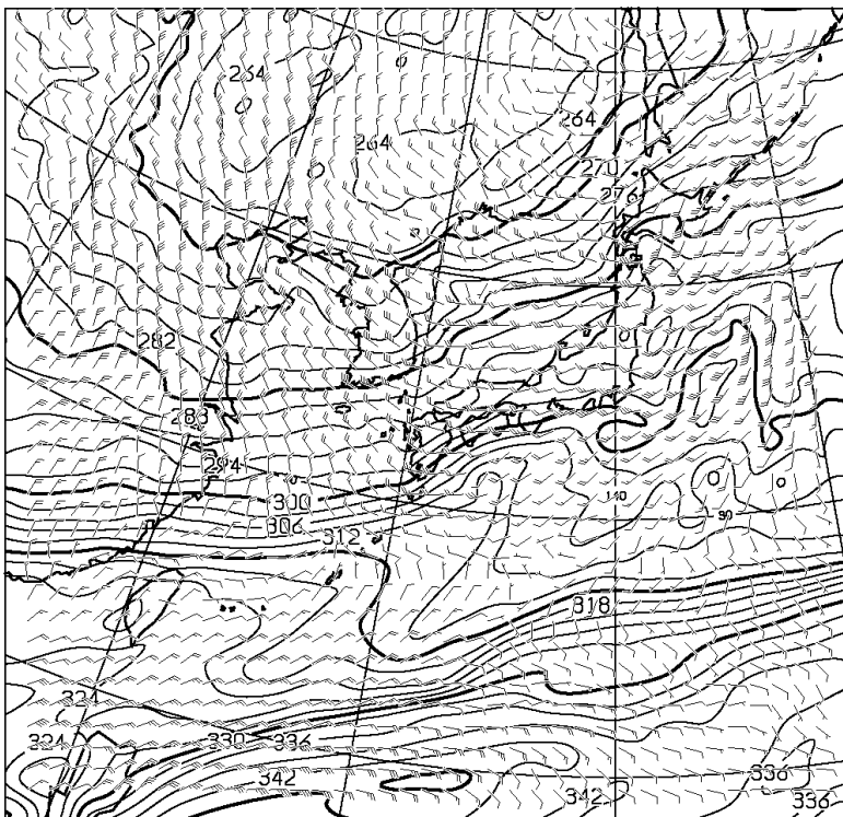
T=36 850hPa: E.P.TEMP(K),WIND(KNOTS) VALID 160000UTC
