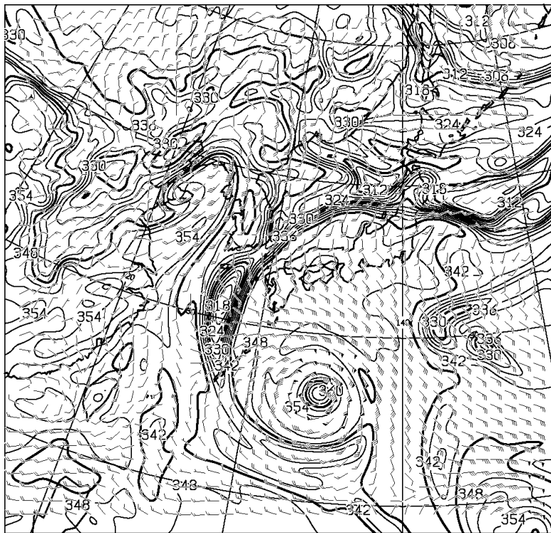
T=12 850hPa: E.P.TEMP(K),WIND(KNOTS) VALID 201200UTC
