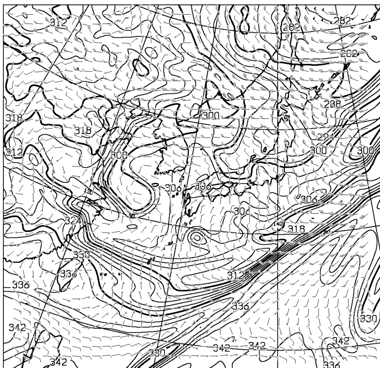
T=36 850hPa: E.P.TEMP(K),WIND(KNOTS) VALID 280000UTC
