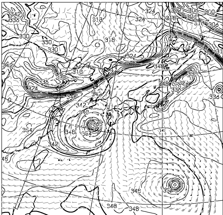
T=48 850hPa: E.P.TEMP(K),WIND(KNOTS) VALID 220000UTC
