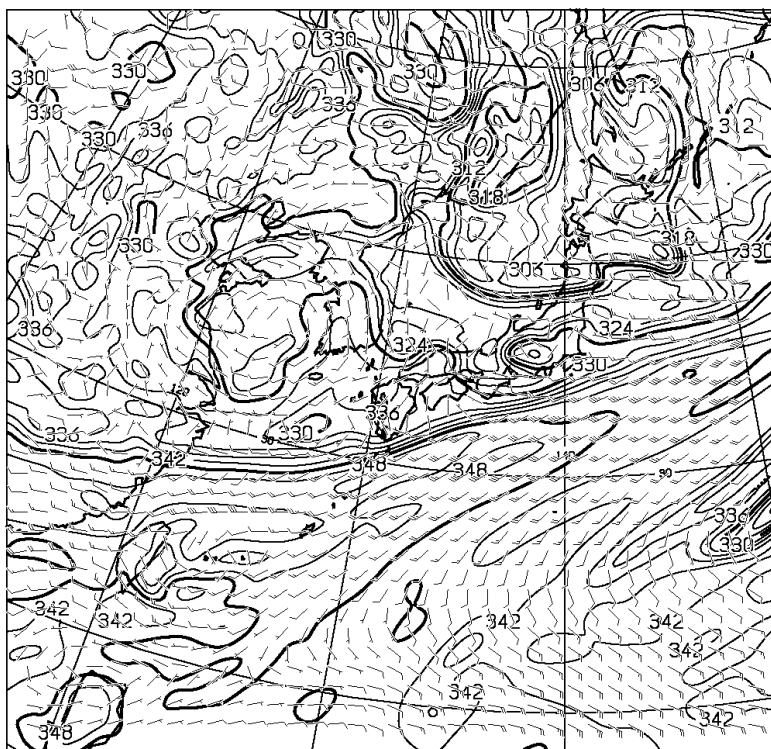
T=36 850hPa: E.P. TEMP(K), WIND(KNOTS) VALID 261200UTC
