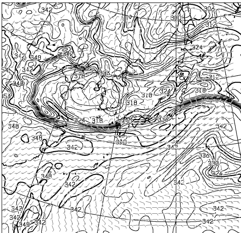
T=24 850hPa: E.P.TEMP(K),WIND(KNOTS) VALID 231200UTC
