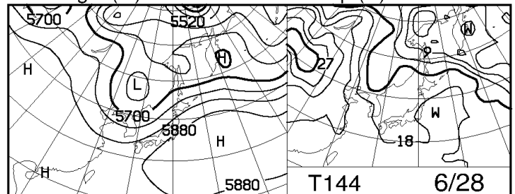
Height (m) at 500hPa
