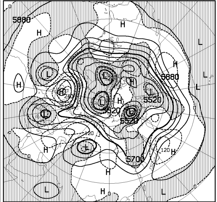
500hPa 5 DAY MEAN Height and Anomaly (m)
