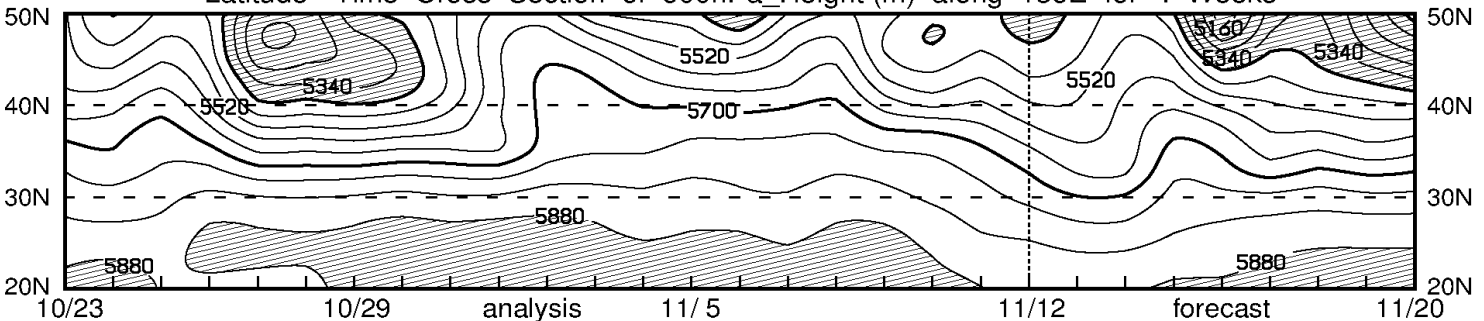
Latitude - Time Cross Section of 500hPa Height (m) along 135E for 4 Weeks
